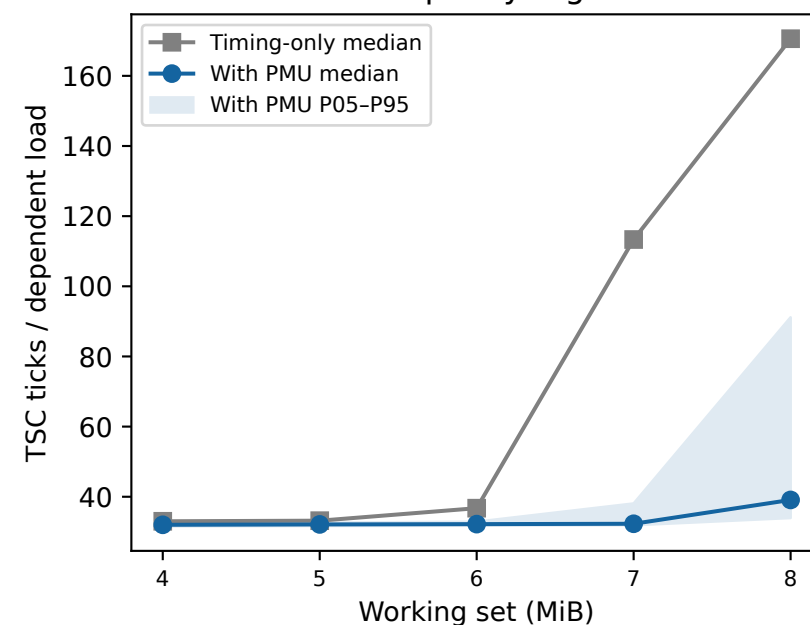
LLC capacity region
