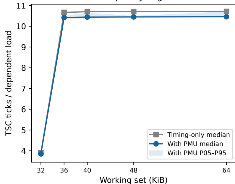
L1 capacity region
