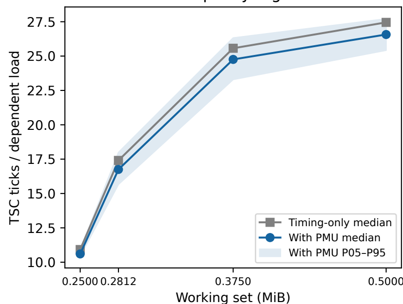
L2 capacity region
