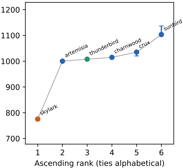
llc loads
