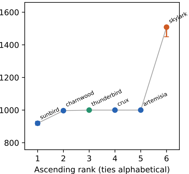
l1 loads
