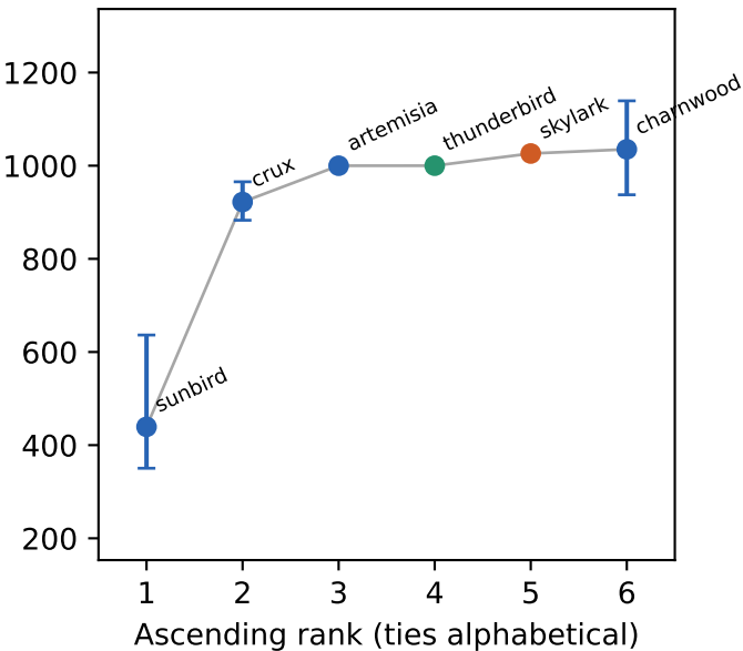
cache misses
