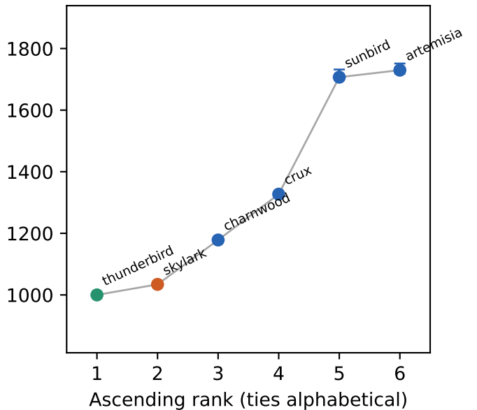
l1 misses
