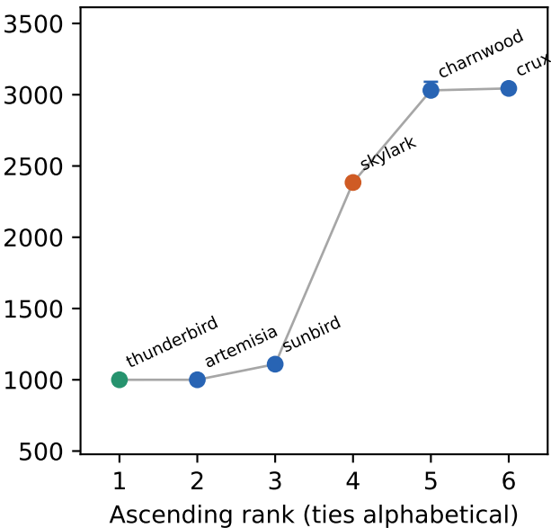
cache references
