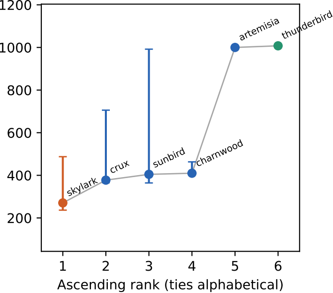
llc misses
