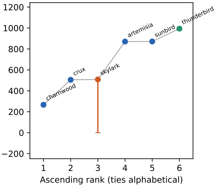
dtlb misses
