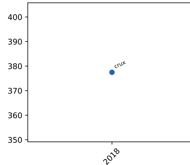
l1c misses
