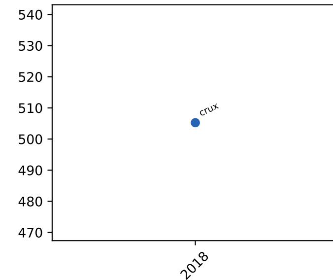
dtlb misses
