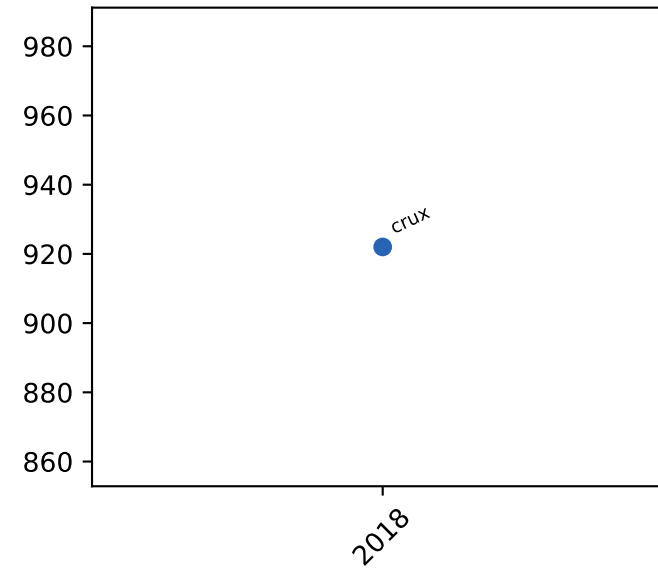
cache misses
