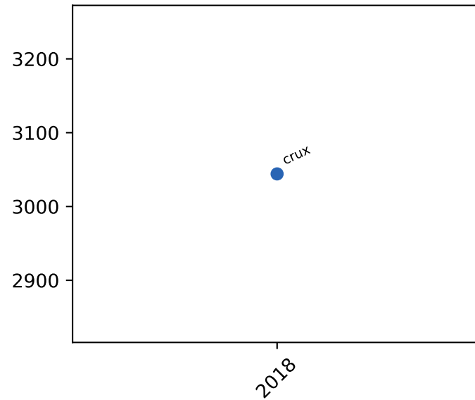
cache references
