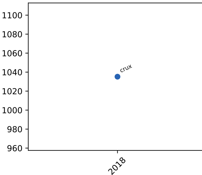
l1c loads
