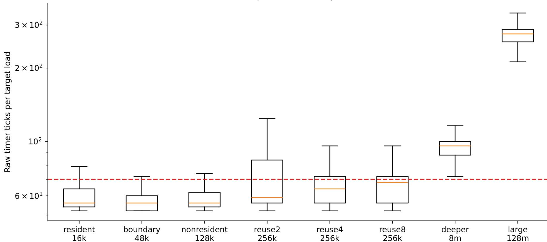
Validation distributions, repeat 1 (1M samples each; 1.5 IQR whiskers)
