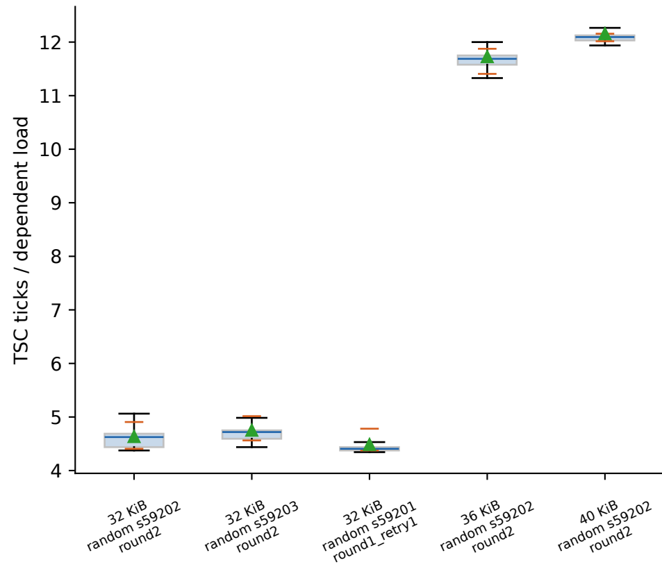
sunbird: L1D
