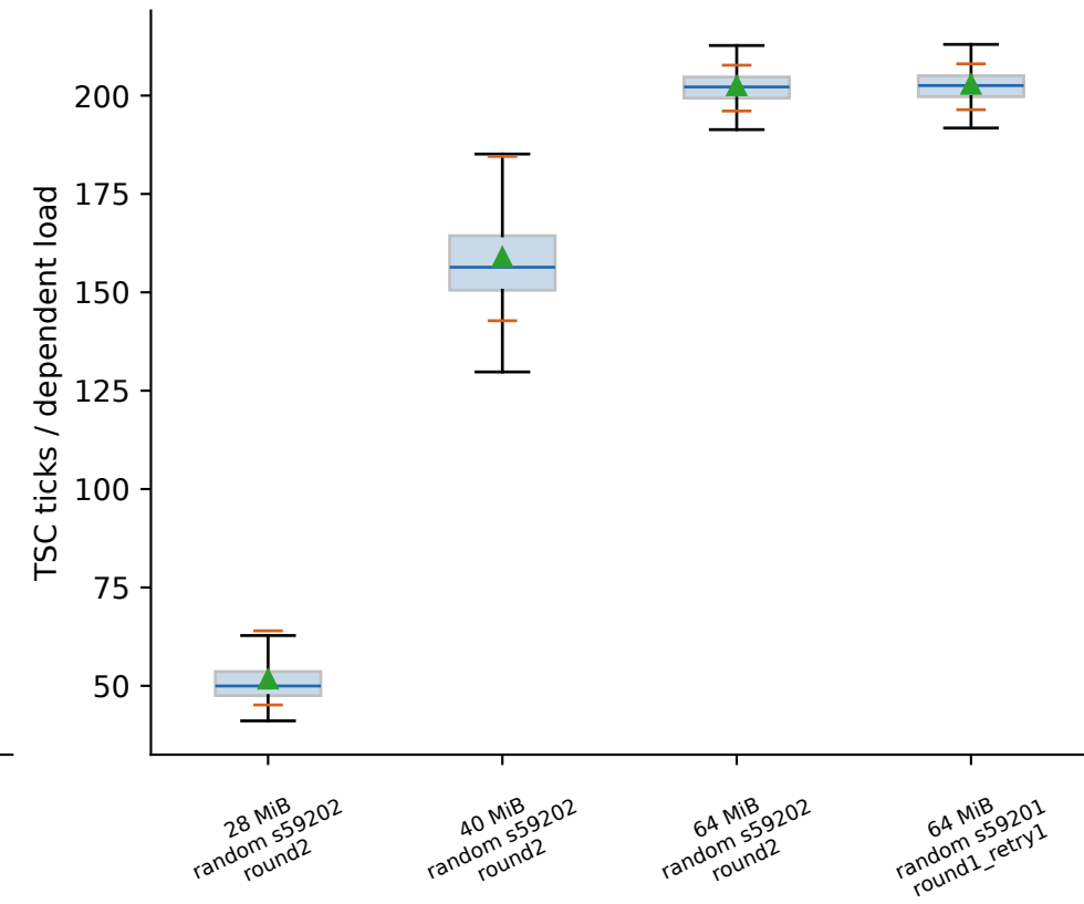
sunbird: LLC effective transition
