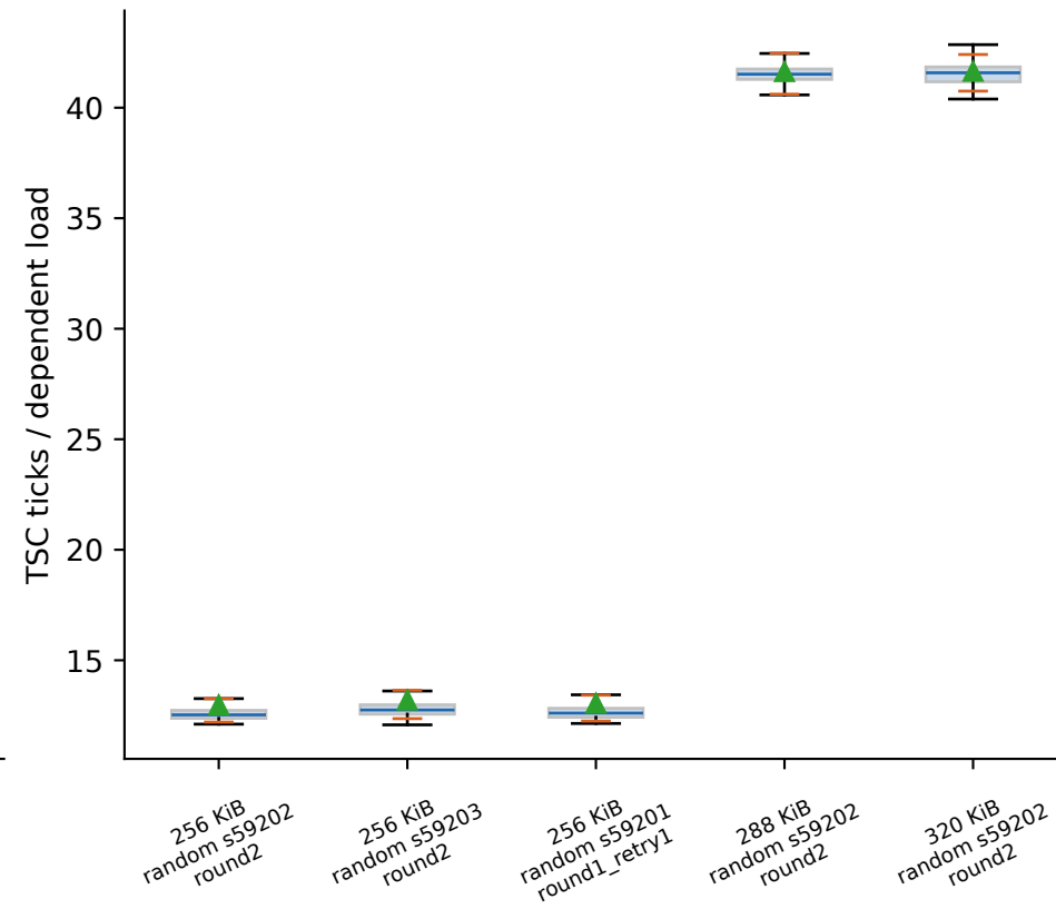
sunbird: L2
