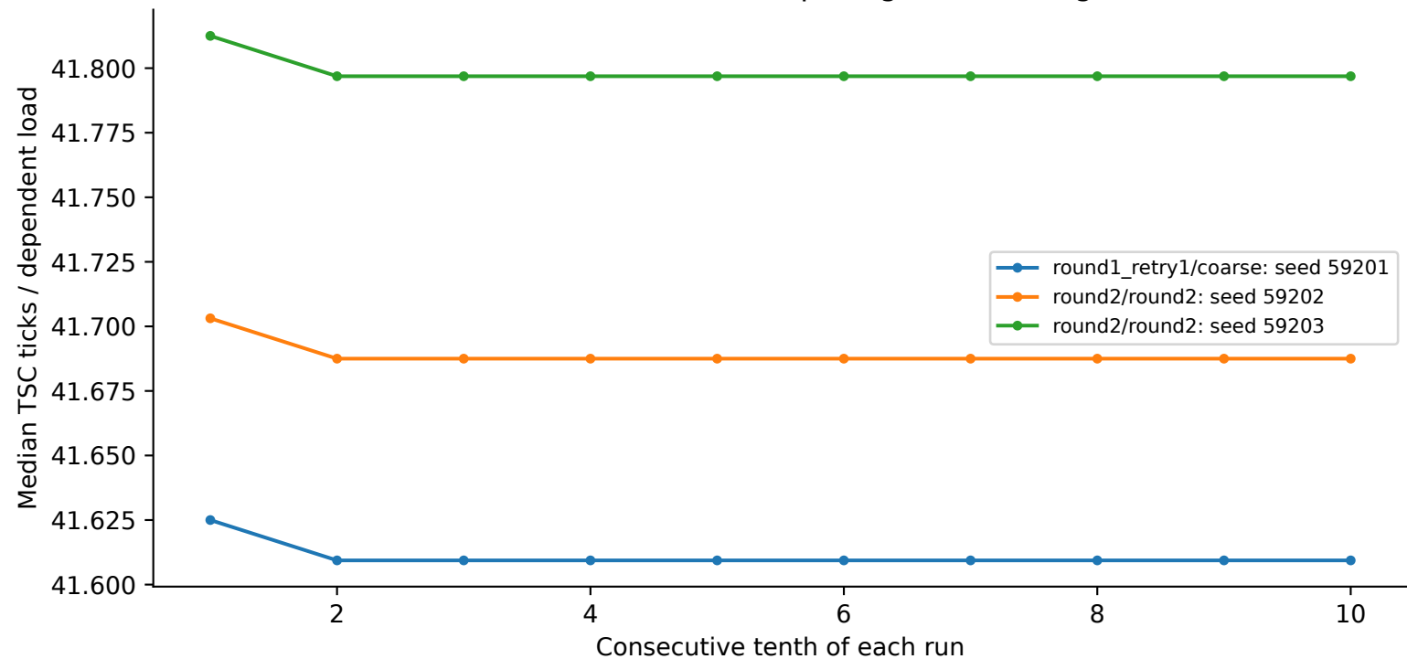
sunbird: 512 KiB, 64 B spacing, N=256, huge
