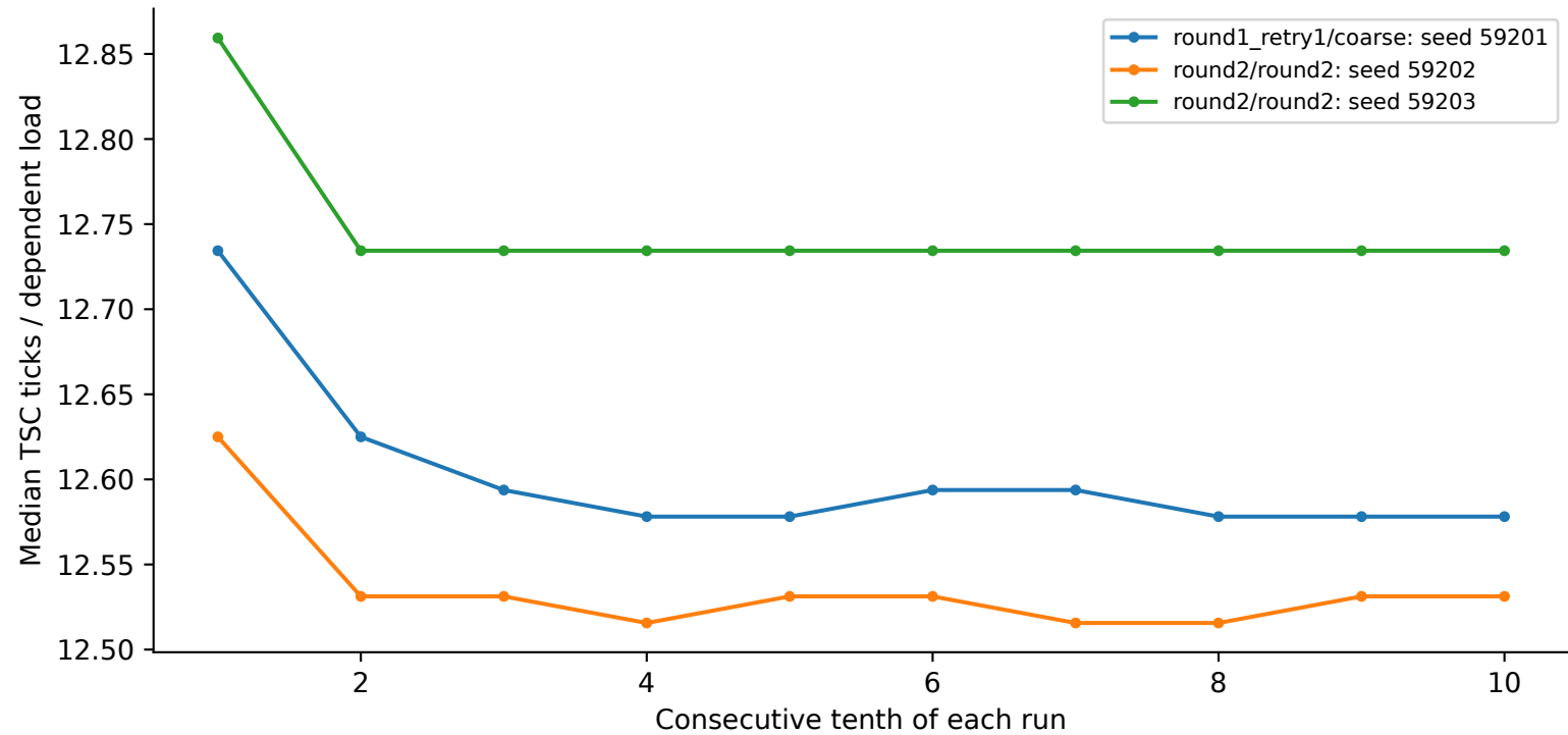
sunbird: 256 KiB, 64 B spacing, N=256, huge
