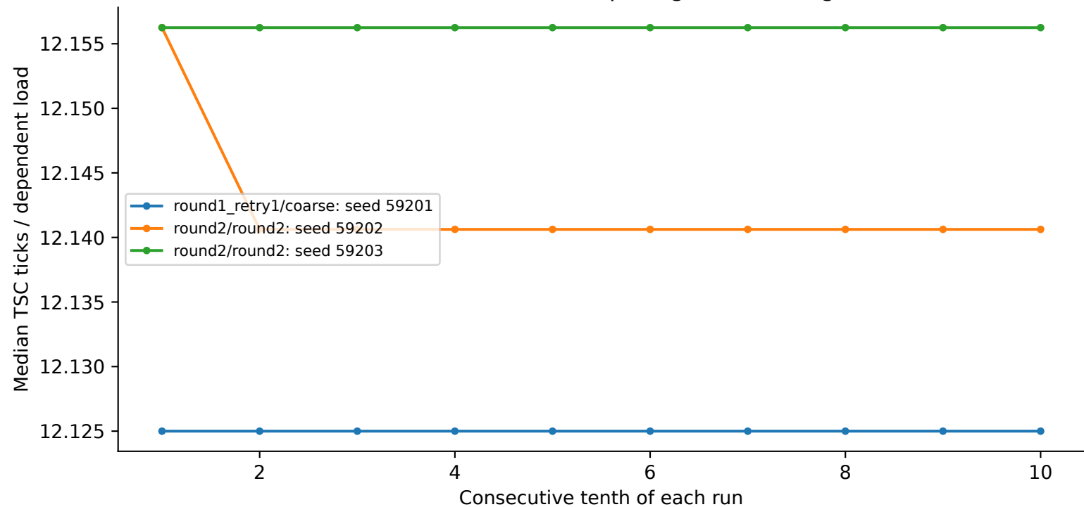
sunbird: 64 KiB, 64 B spacing, N=256, huge
