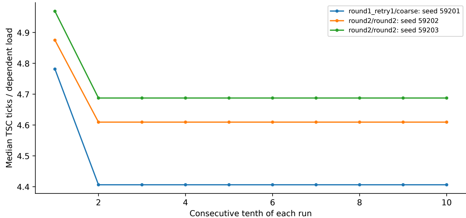
sunbird: 32 KiB, 64 B spacing, N=256, huge
