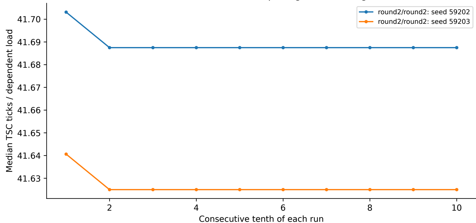
sunbird: 384 KiB, 64 B spacing, N=256, huge
