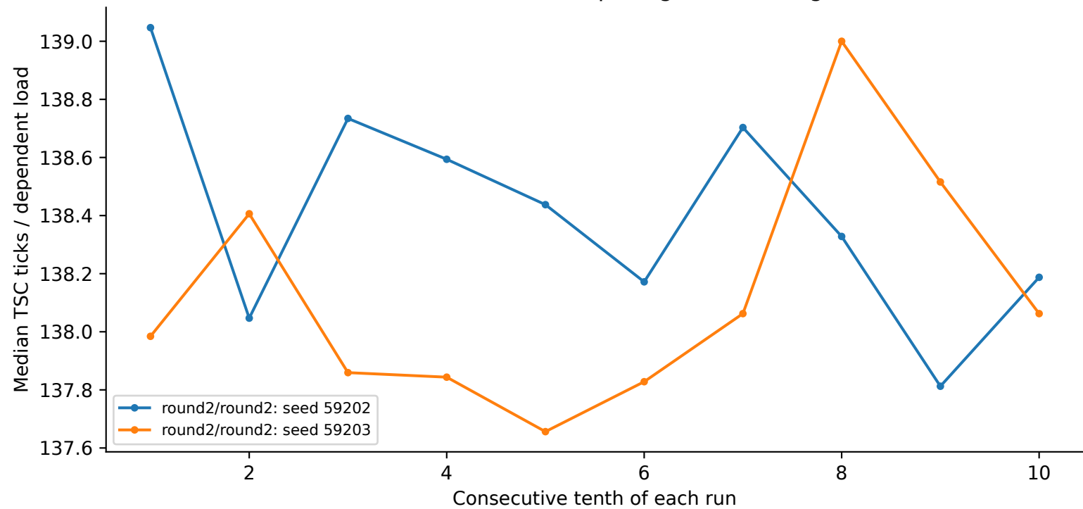
sunbird: 64 MiB, 8 B spacing, N=256, huge
