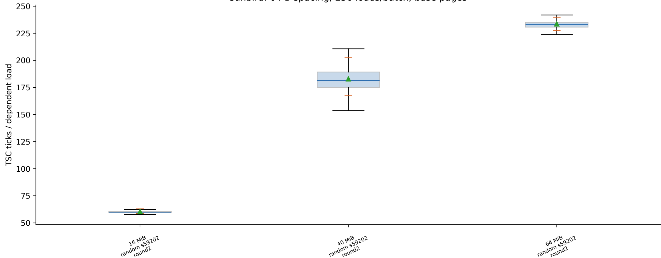
sunbird: 64 B spacing, 256 loads/batch, base pages
