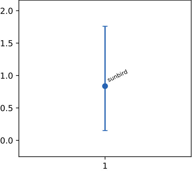
l1 misses
