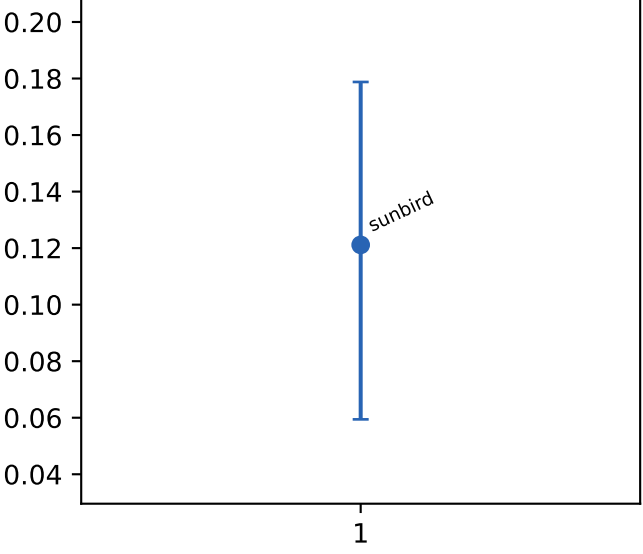
l1c loads
