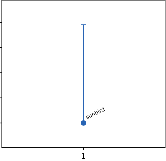
cache misses
