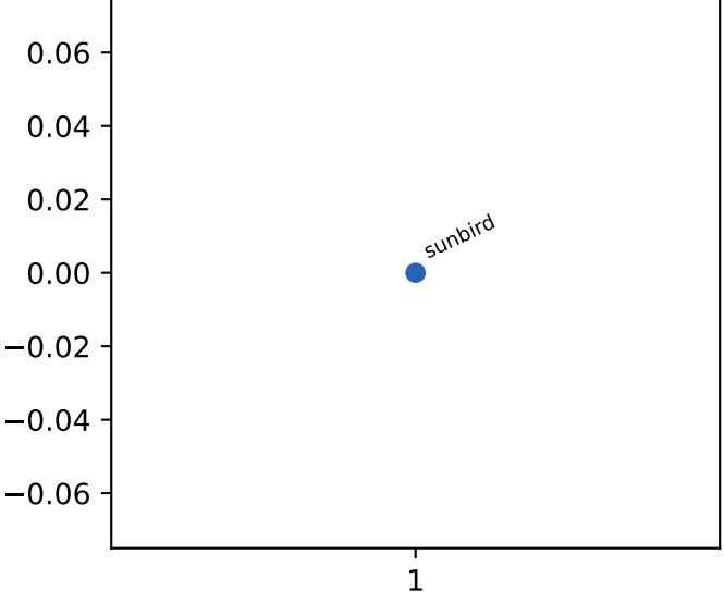
l1c misses
