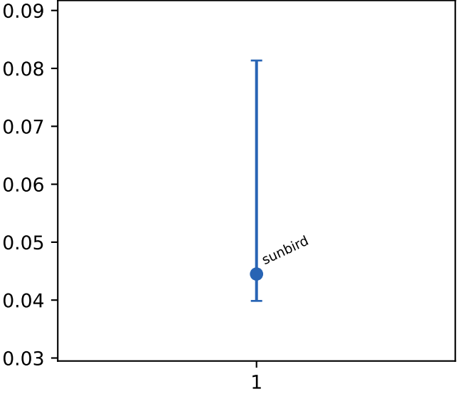
l1 loads
