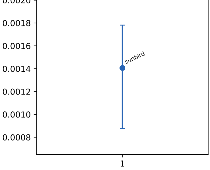
dtlb misses
