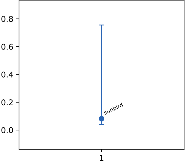
cache references
