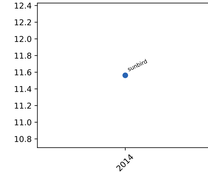
l1 misses
