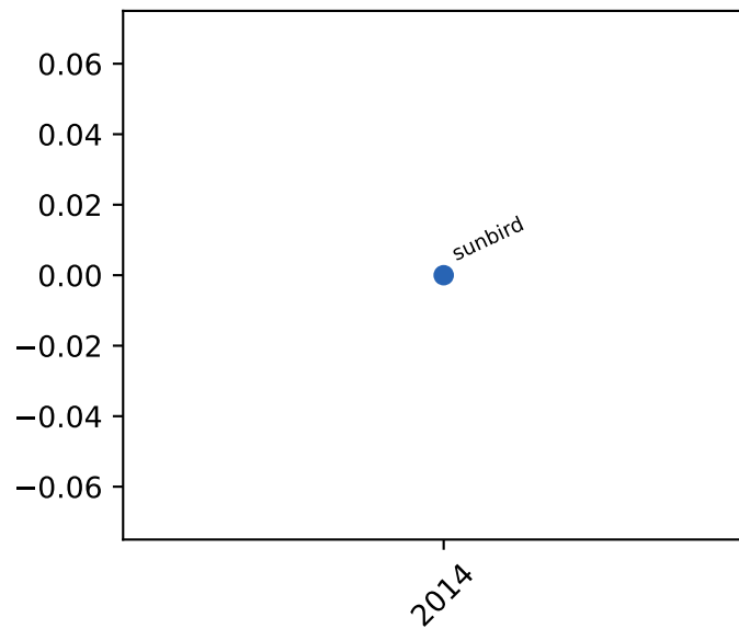
l1c misses
