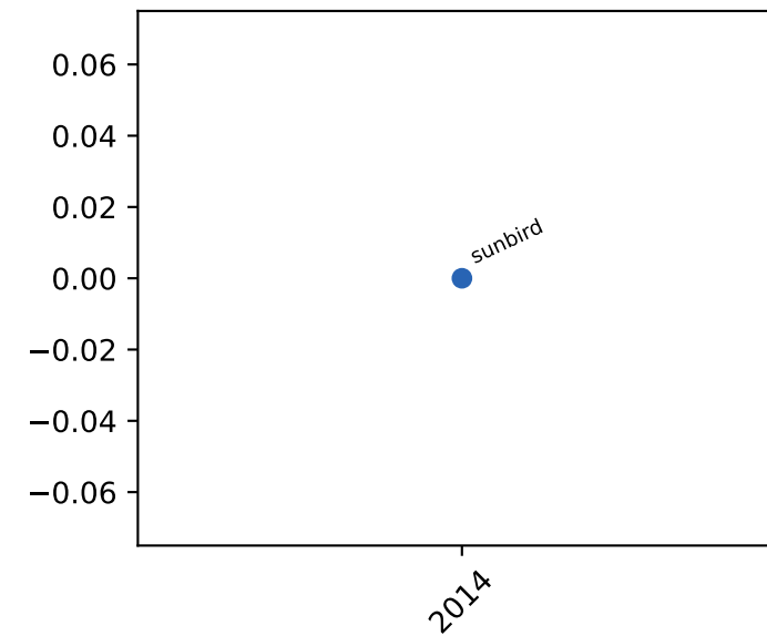
dtlb misses
