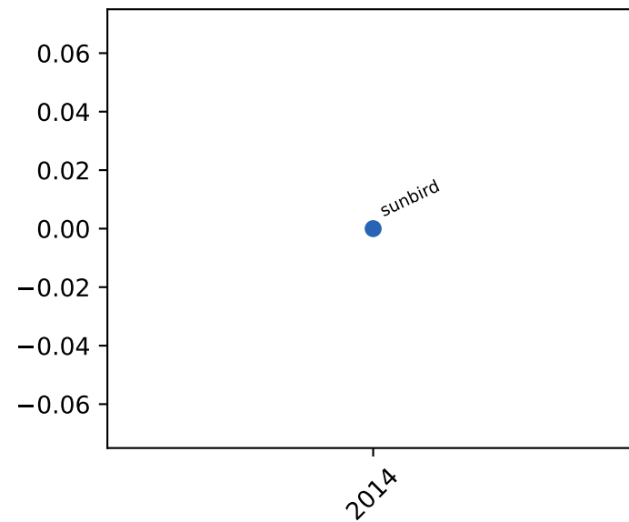
cache misses
