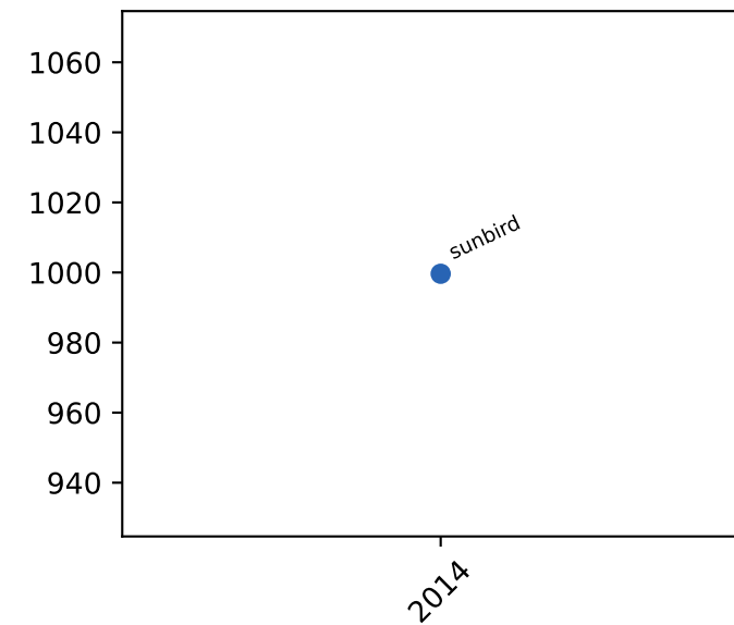
l1 loads
