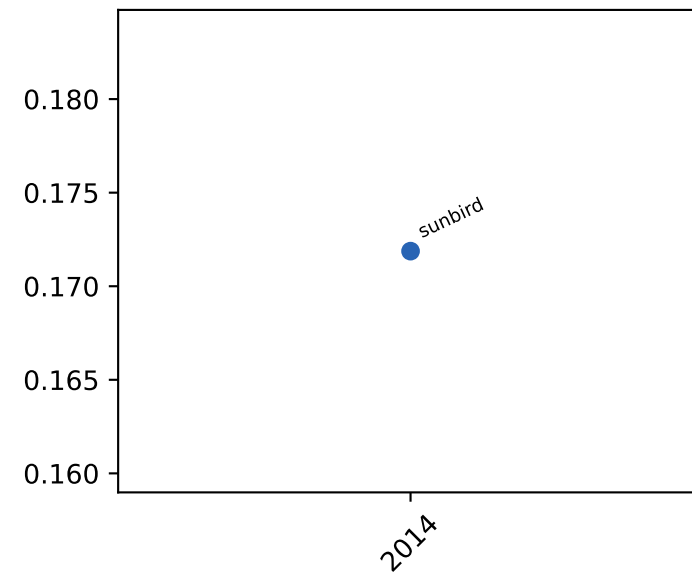
l1c loads
