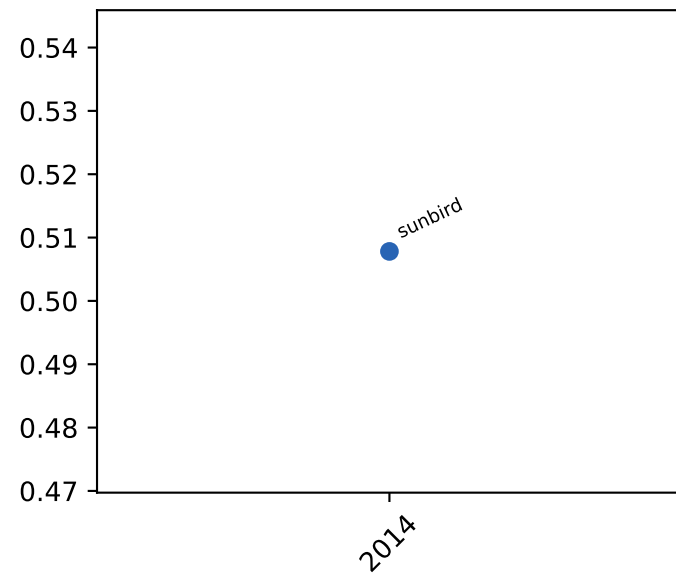
cache references
