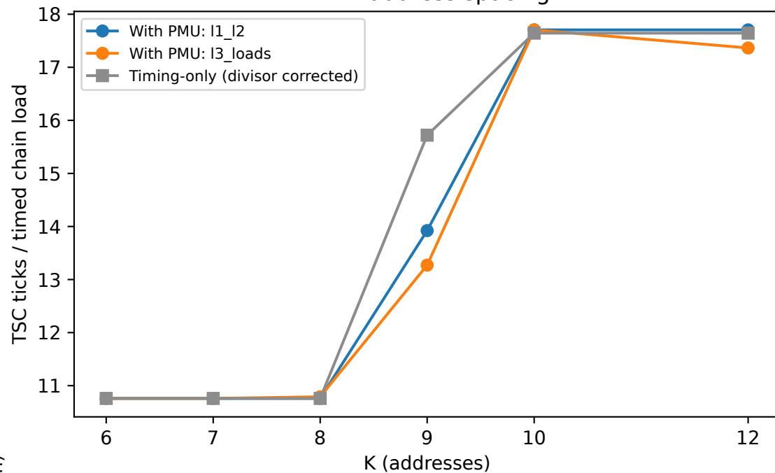
4 KiB address spacing
