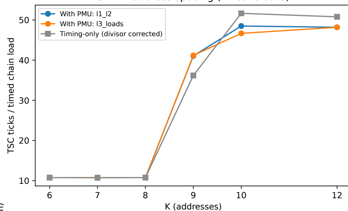
32 KiB address spacing (L2 candidate)
