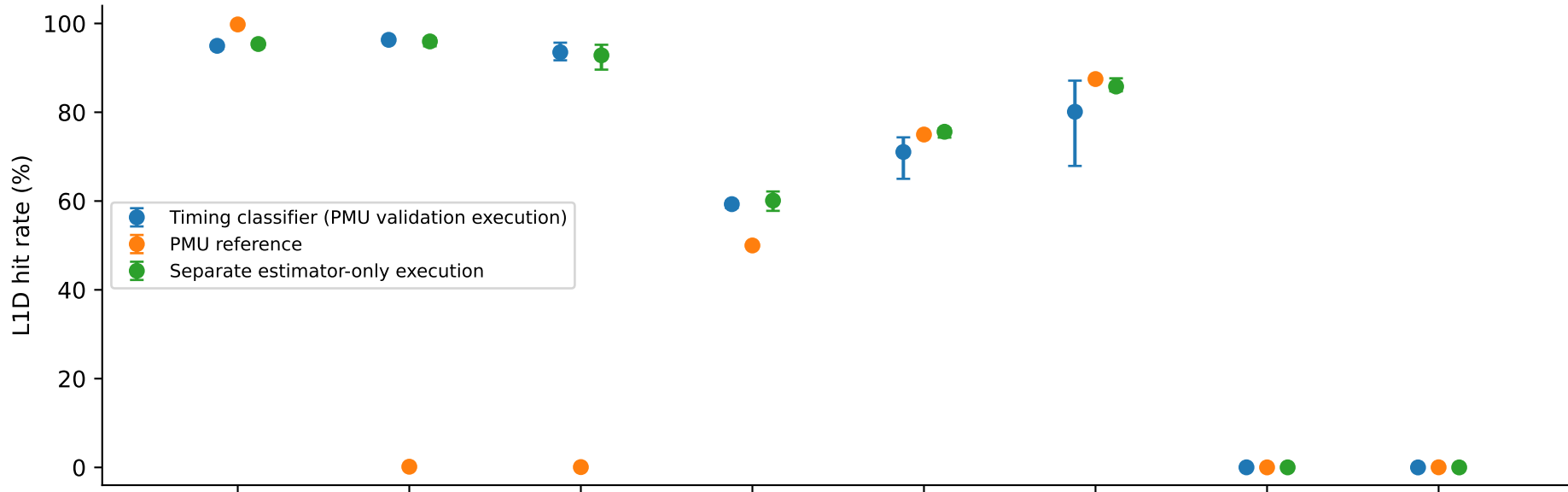
Frozen classifier versus PMU (mean and range of three repeats)
