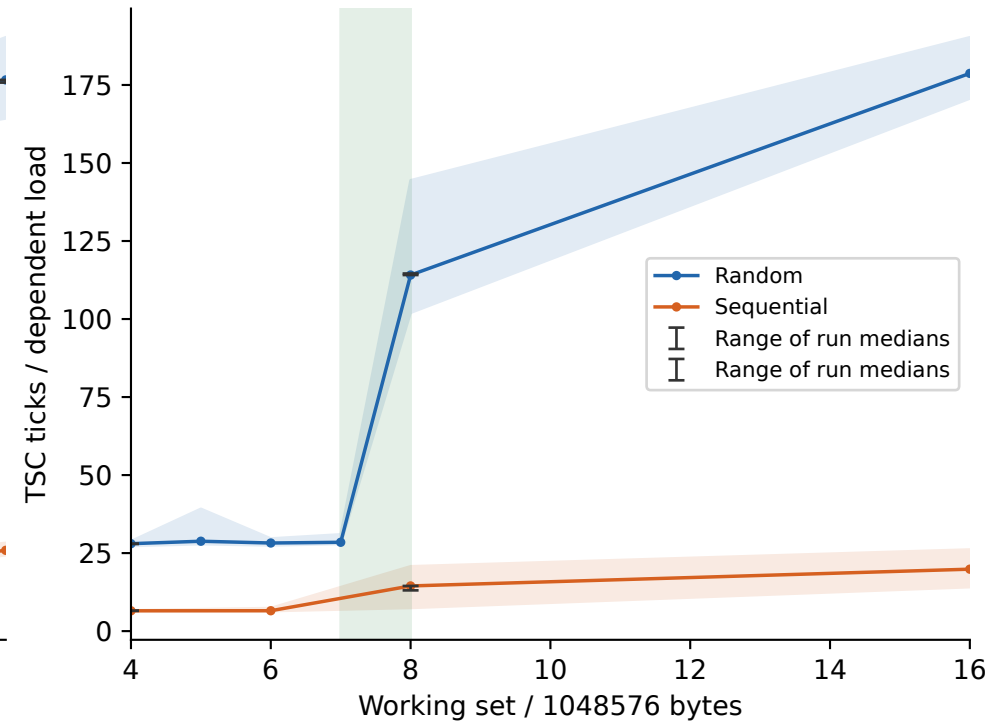
upgrade: LLC effective transition
