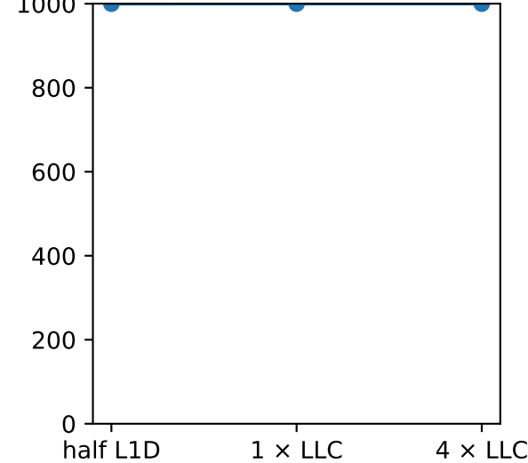
LLC-load-misses
