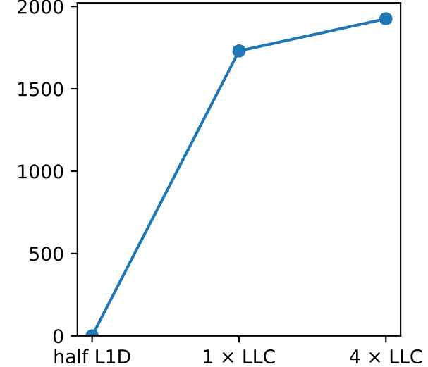
dTLB-load-misses
