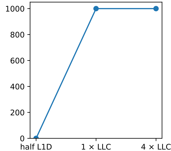
LLC-load-misses
