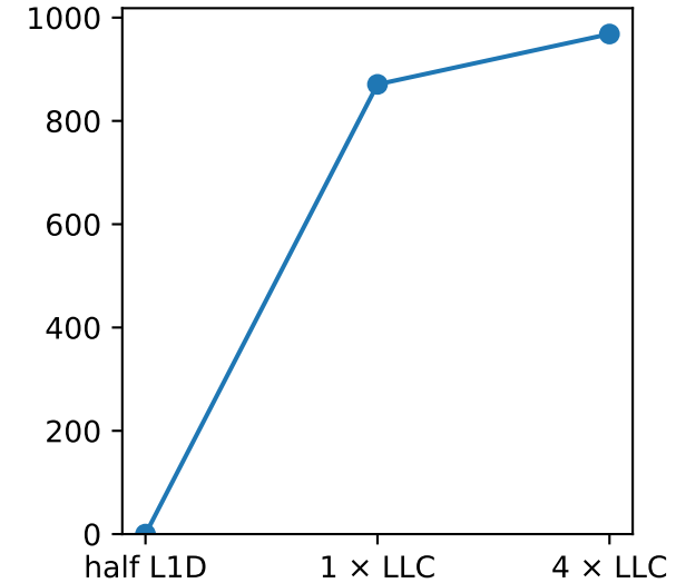
dTLB-load-misses
