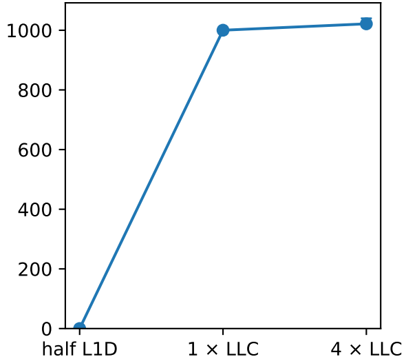
L1-dcache-stores
