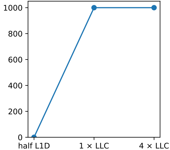
LLC-loads
