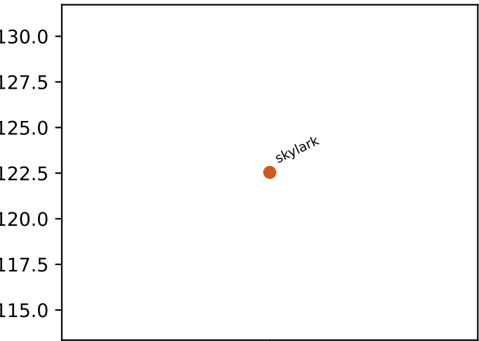
llc loads
