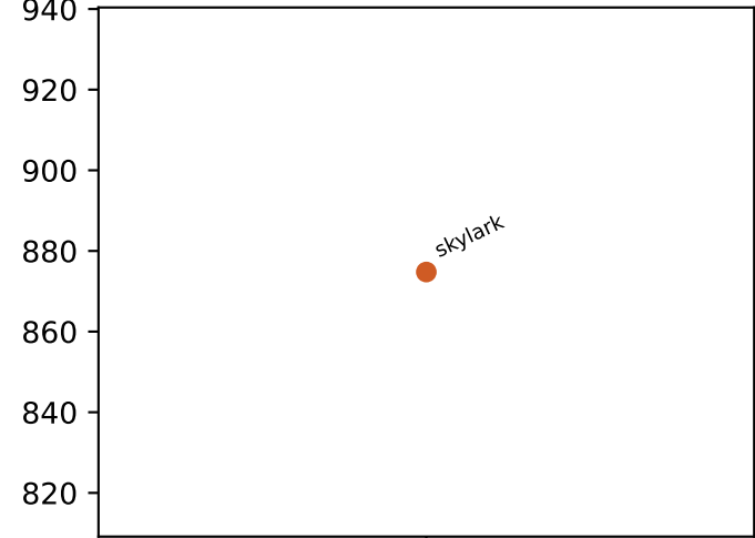
llc misses
