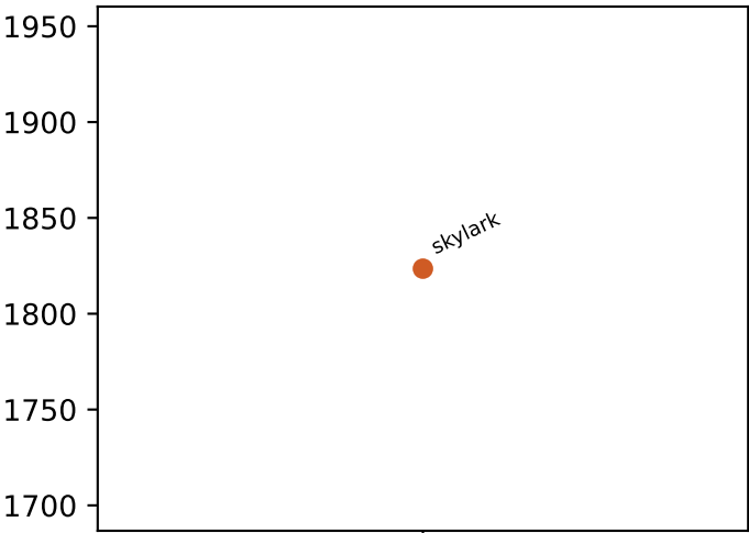
l1 loads
