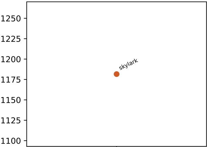
cache misses
