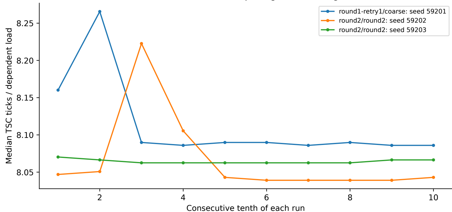
crux: 256 KiB, 64 B spacing, N=256, huge
