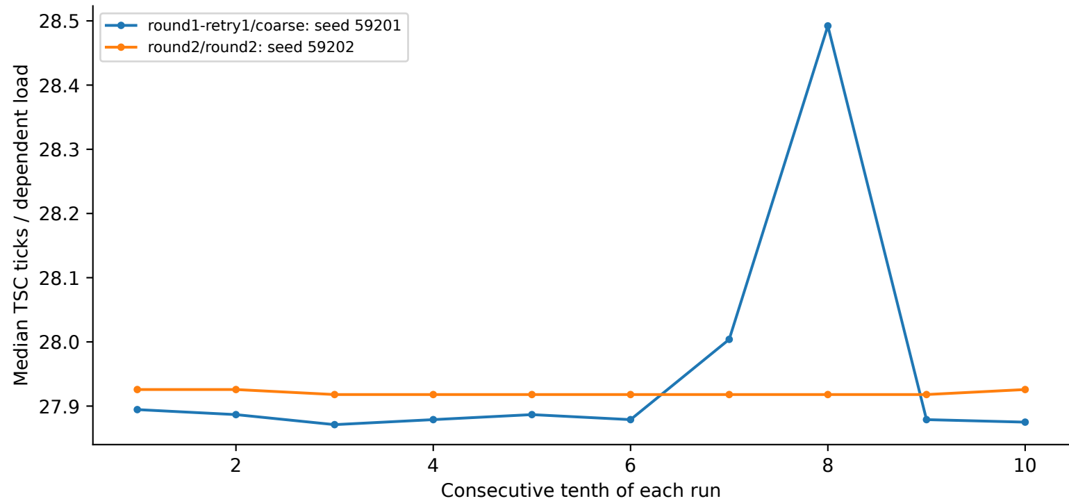
crux: 4 MiB, 64 B spacing, N=256, huge
