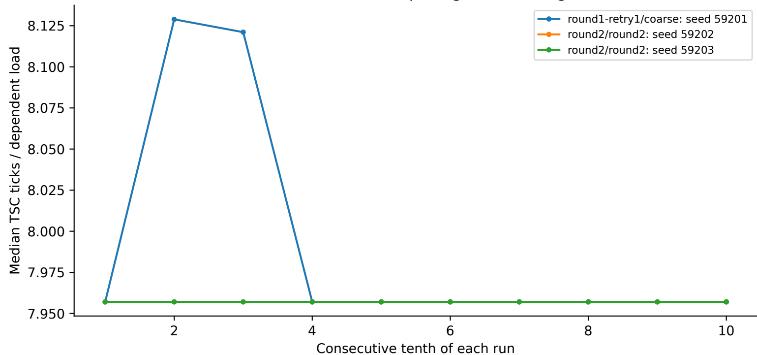
crux: 64 KiB, 64 B spacing, N=256, huge
