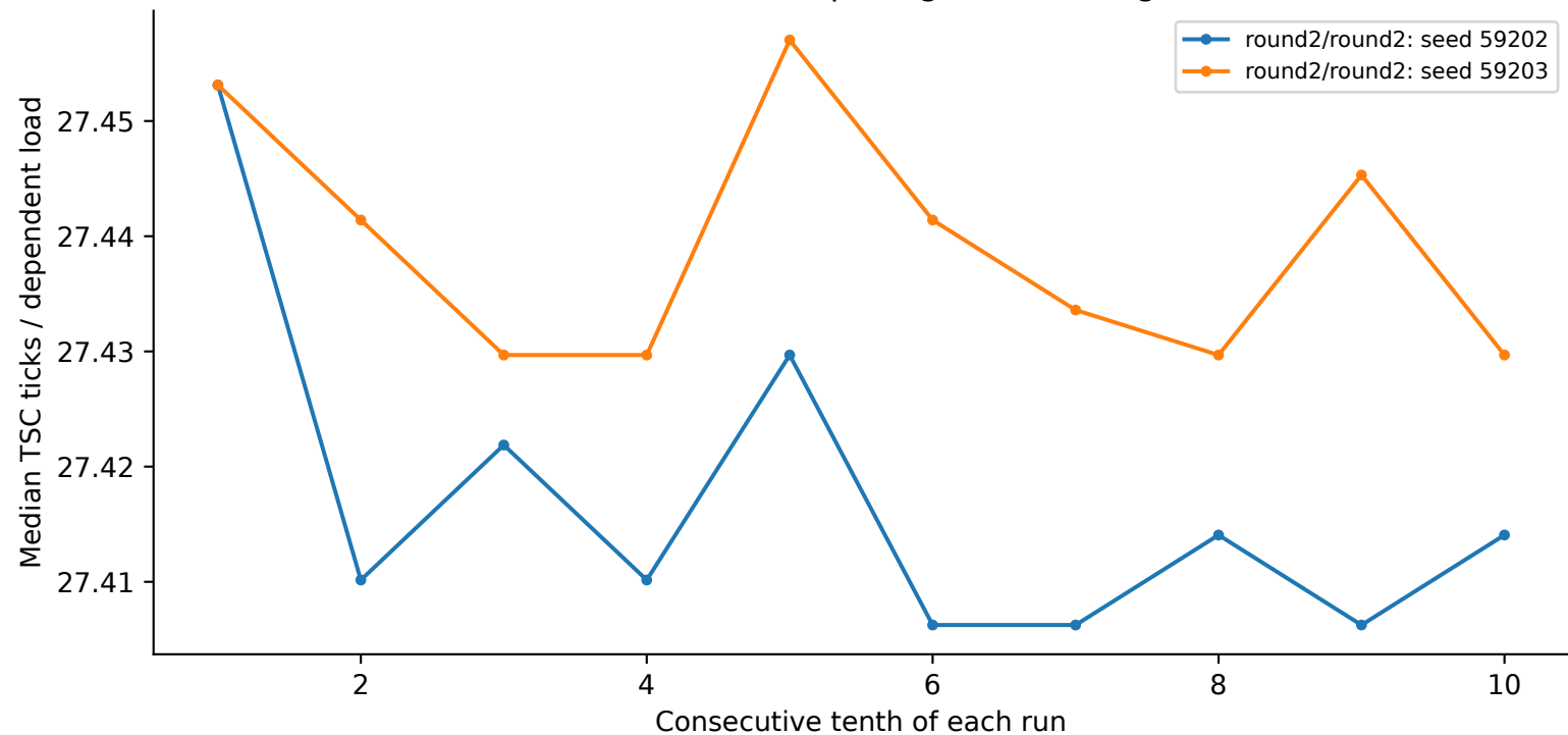
crux: 4 MiB, 8 B spacing, N=256, huge
