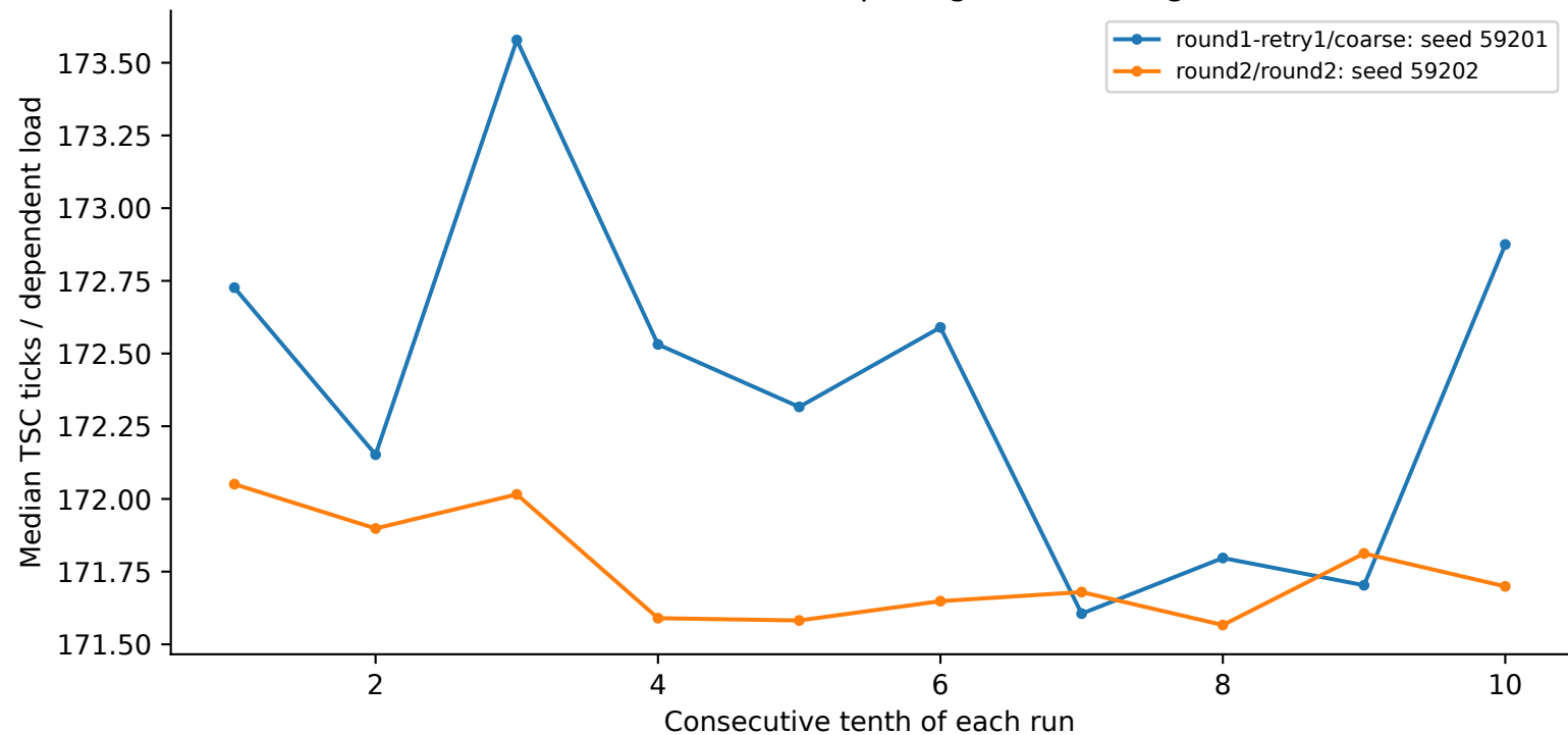
crux: 16 MiB, 64 B spacing, N=256, huge
