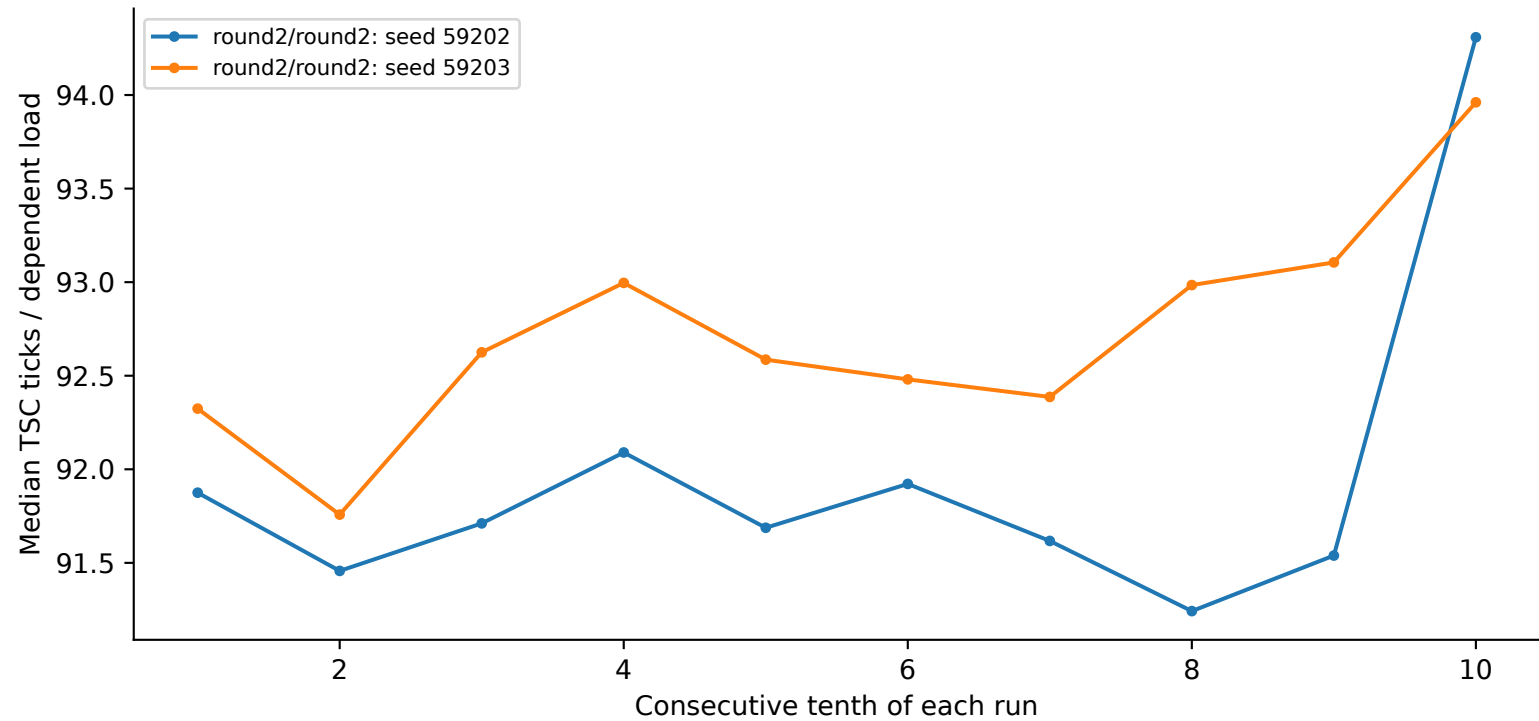
crux: 10 MiB, 8 B spacing, N=256, huge
