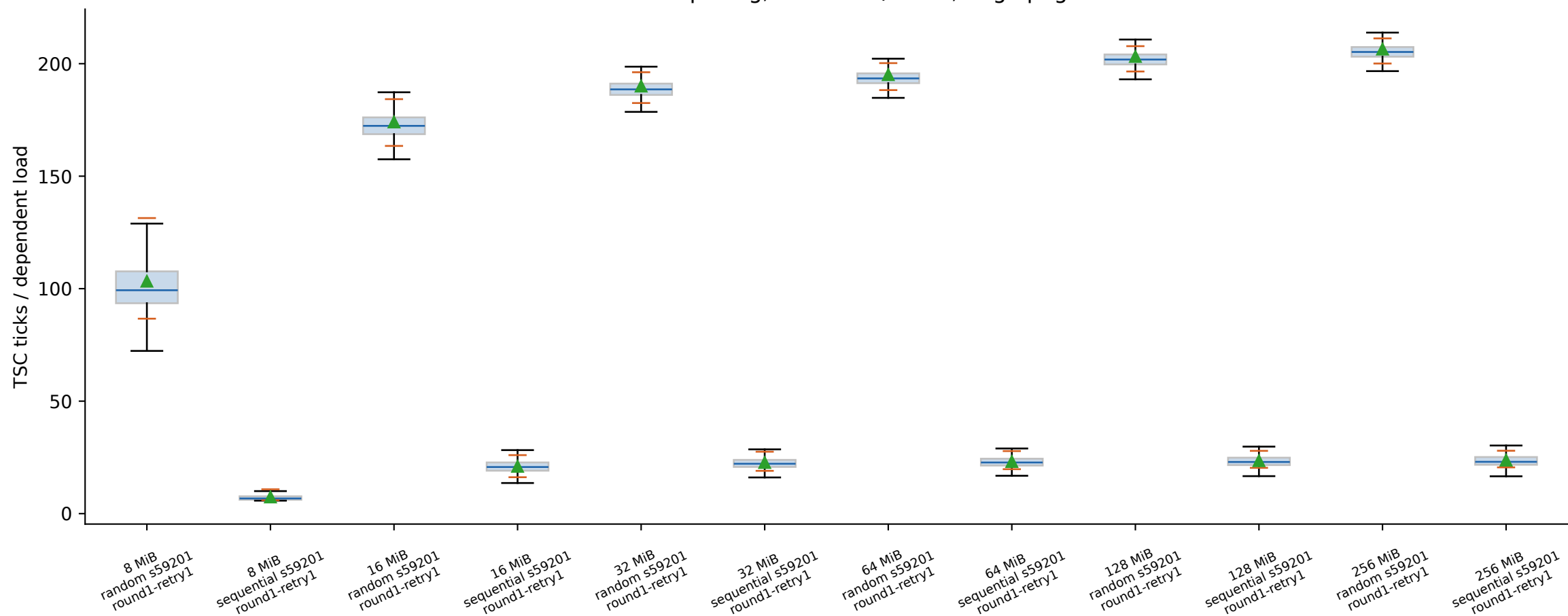
crux: 64 B spacing, 256 loads/batch, huge pages
