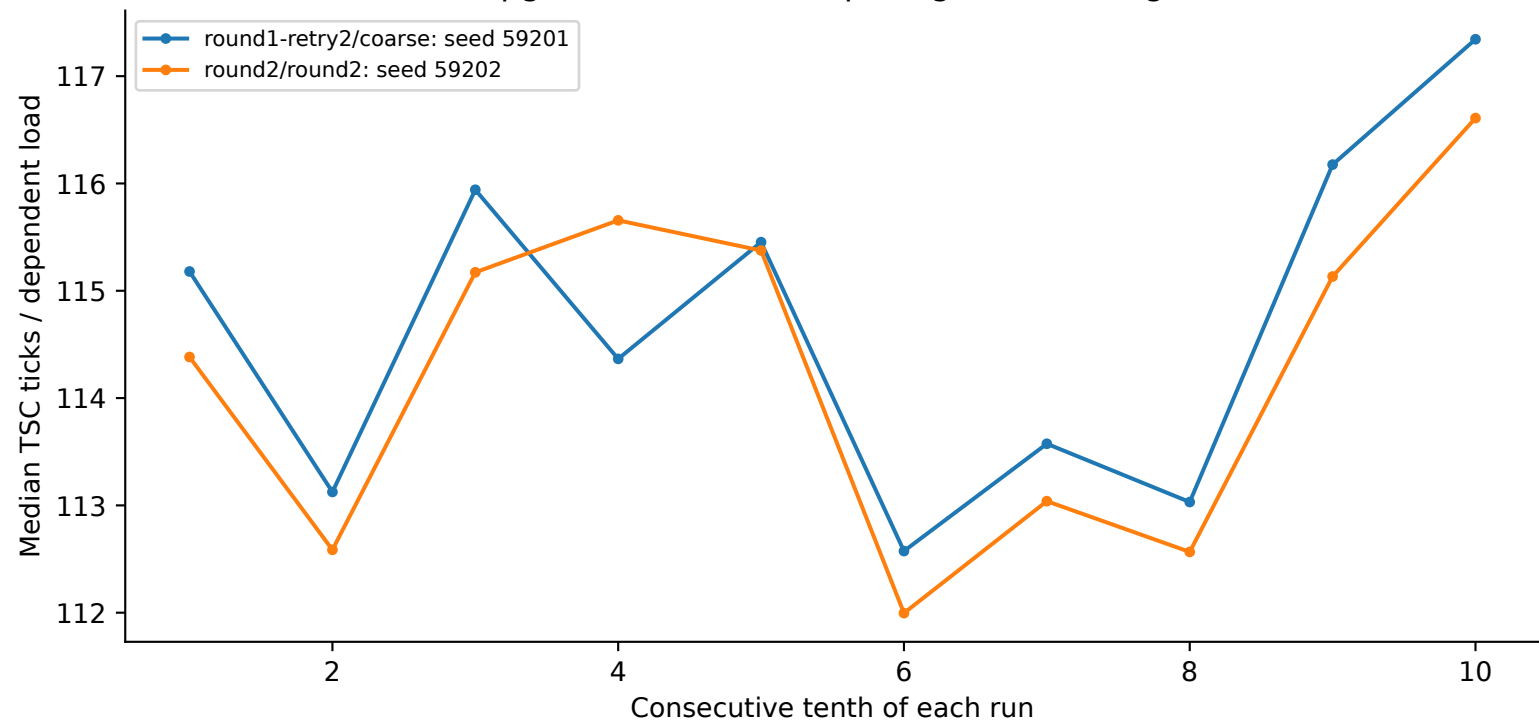
upgrade: 8 MiB, 64 B spacing, N=256, huge
