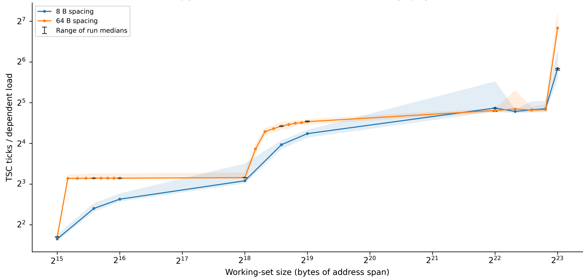
upgrade: random chains, 256 loads/batch, huge pages
