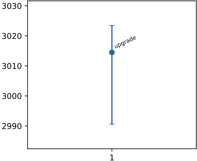
cache references
