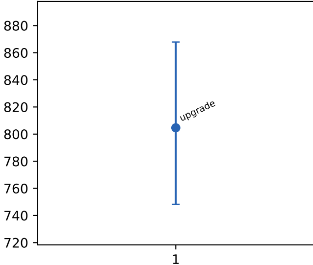
cache misses
