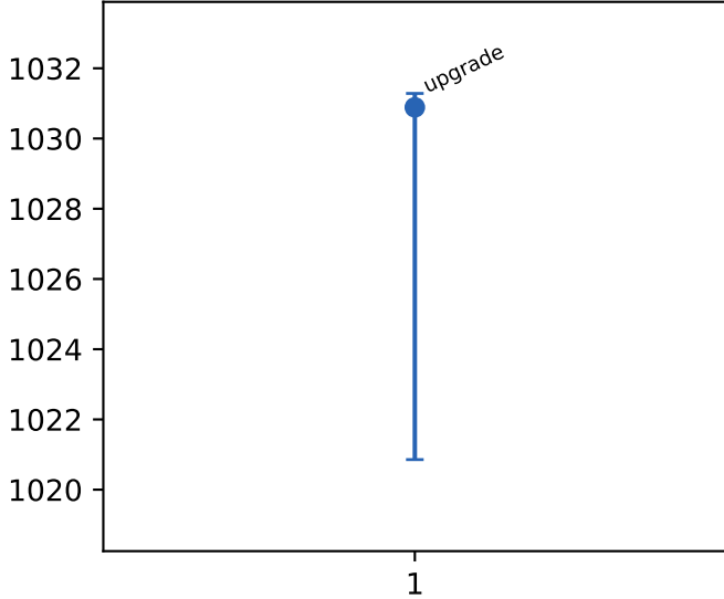
l1c loads
