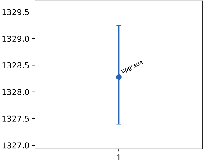
l1 misses
