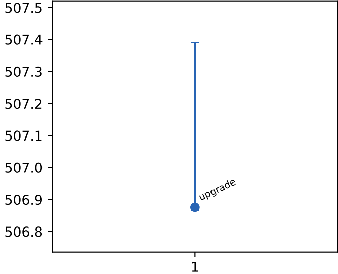
dtlb misses
