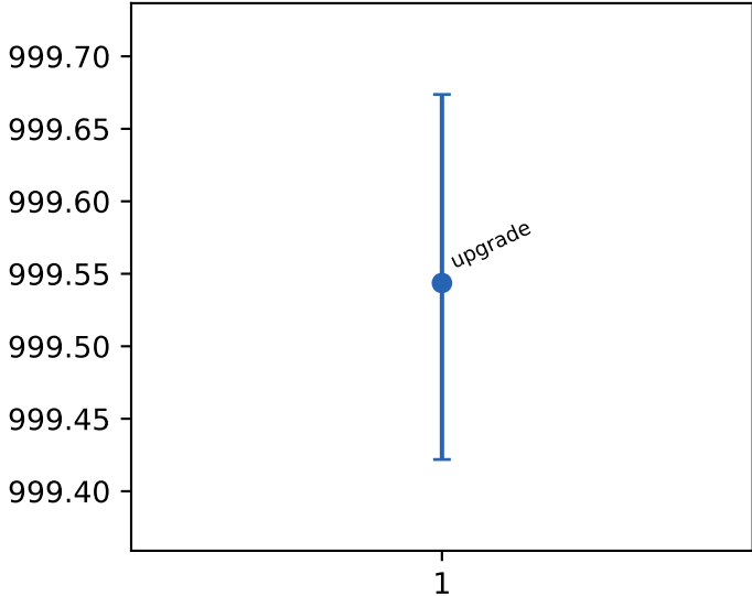
l1 loads
