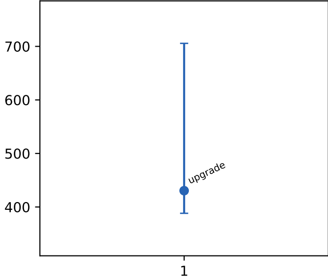
l1c misses
