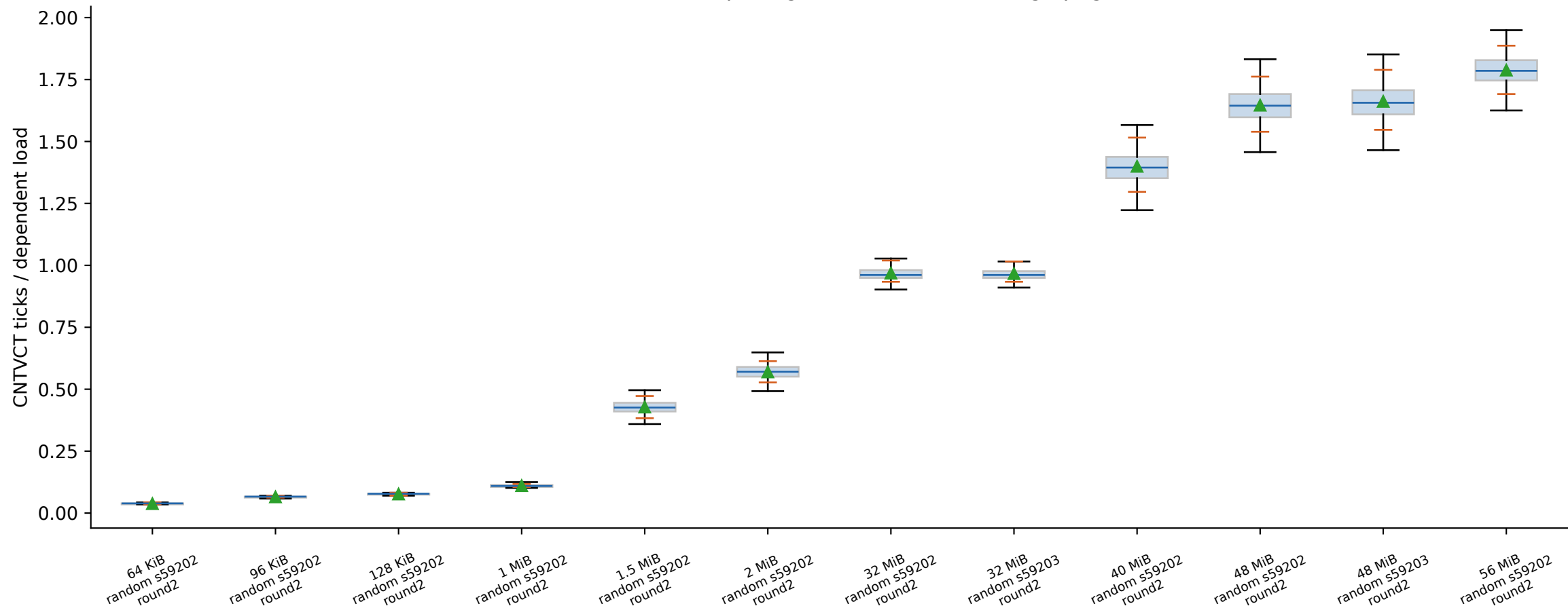
thunderbird: 8 B spacing, 256 loads/batch, huge pages
