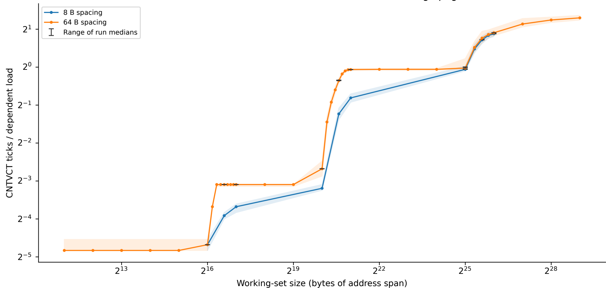
thunderbird: random chains, 256 loads/batch, huge pages
