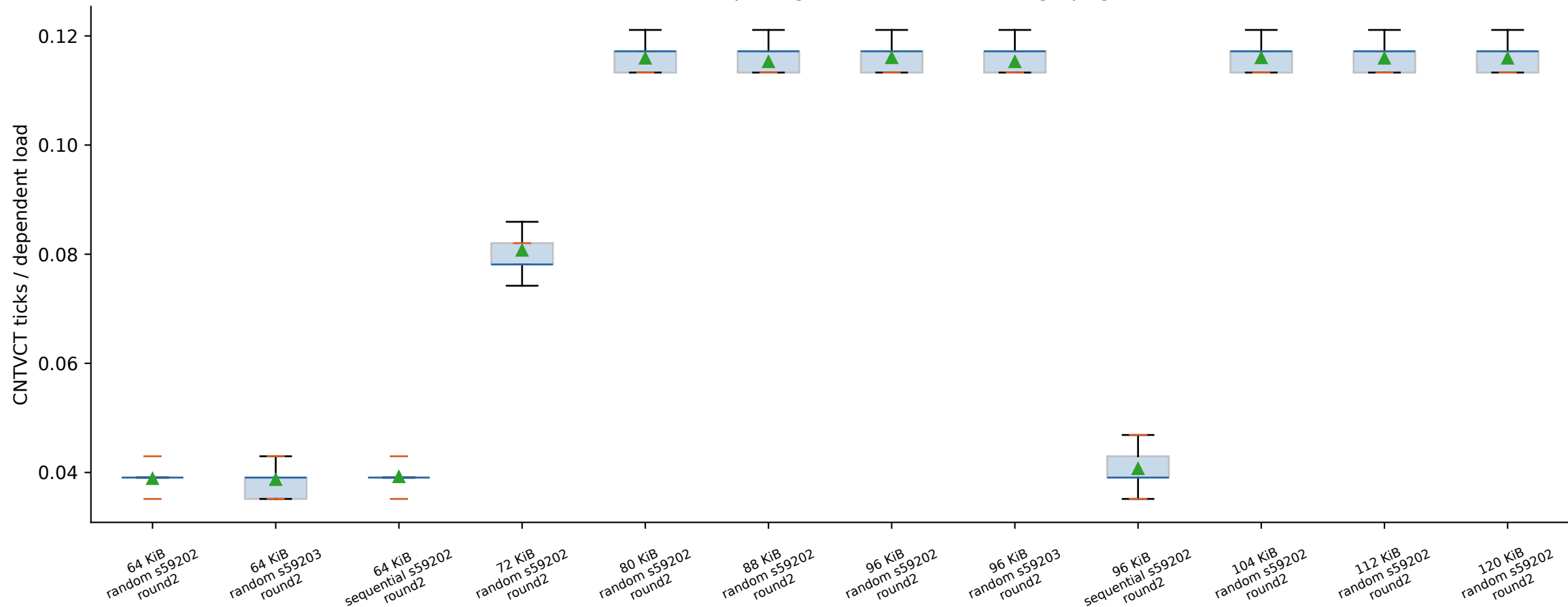
thunderbird: 64 B spacing, 256 loads/batch, huge pages
