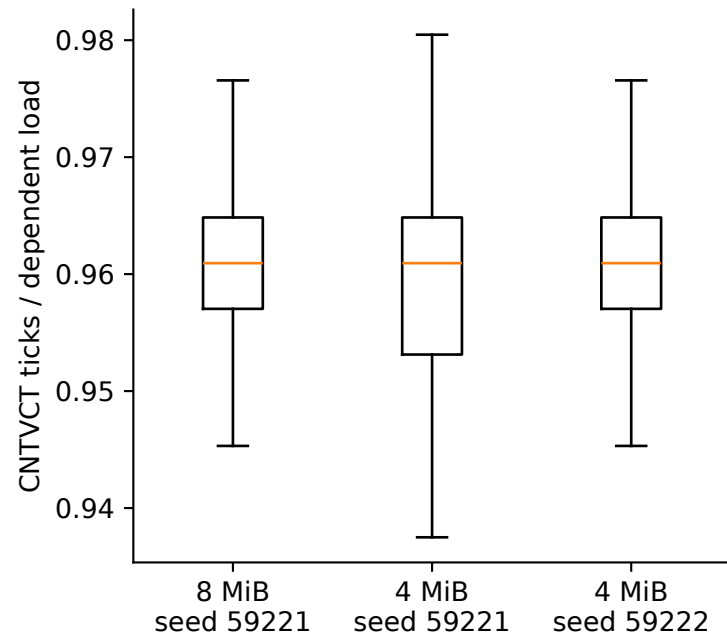
LLC resident candidate
