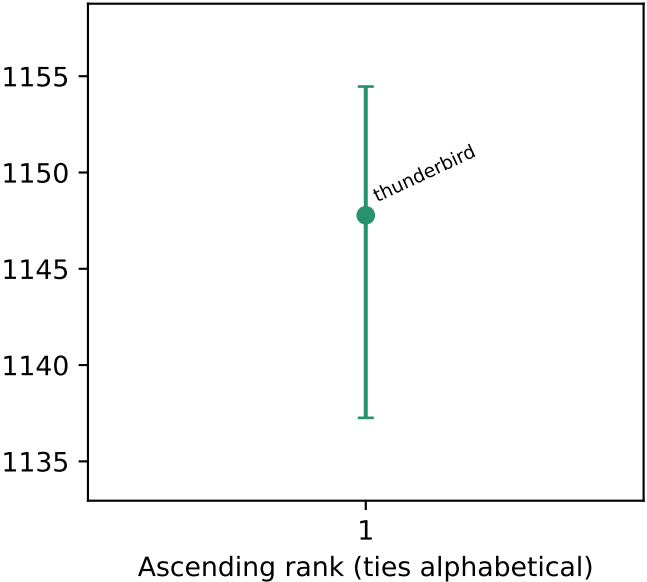
llc loads
