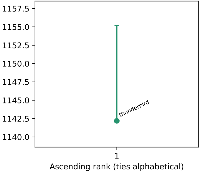
llc misses
