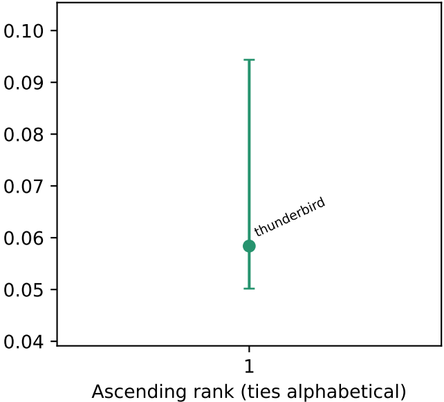
dtlb misses
