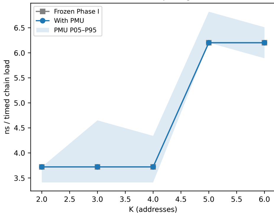
L1 (16 KiB spacing)
