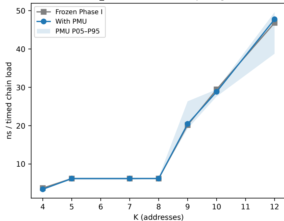
L2_candidate (128 KiB spacing)
