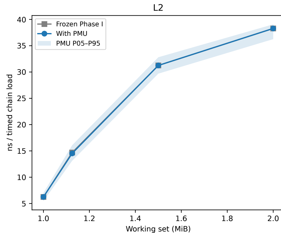
Thunderbird capacity: identical Phase-I workloads, four simultaneous user PMU events
