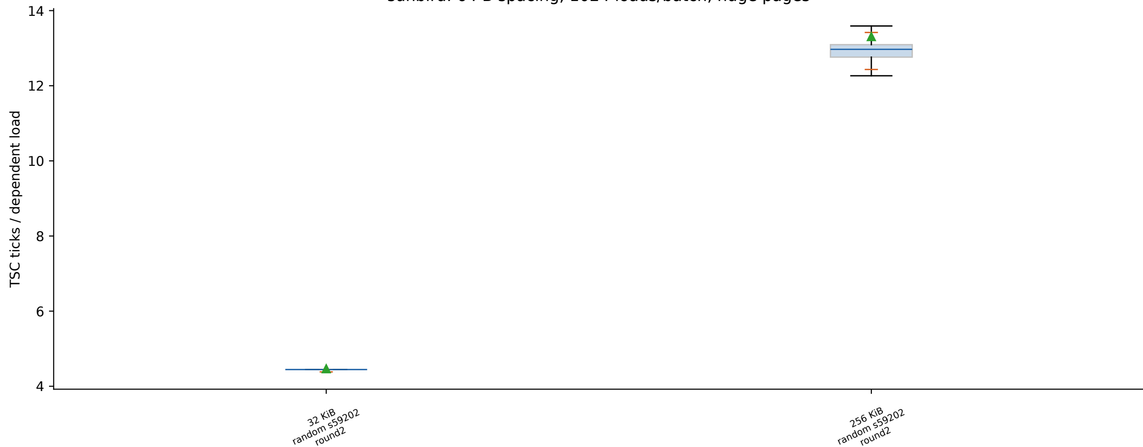
sunbird: 64 B spacing, 1024 loads/batch, huge pages
