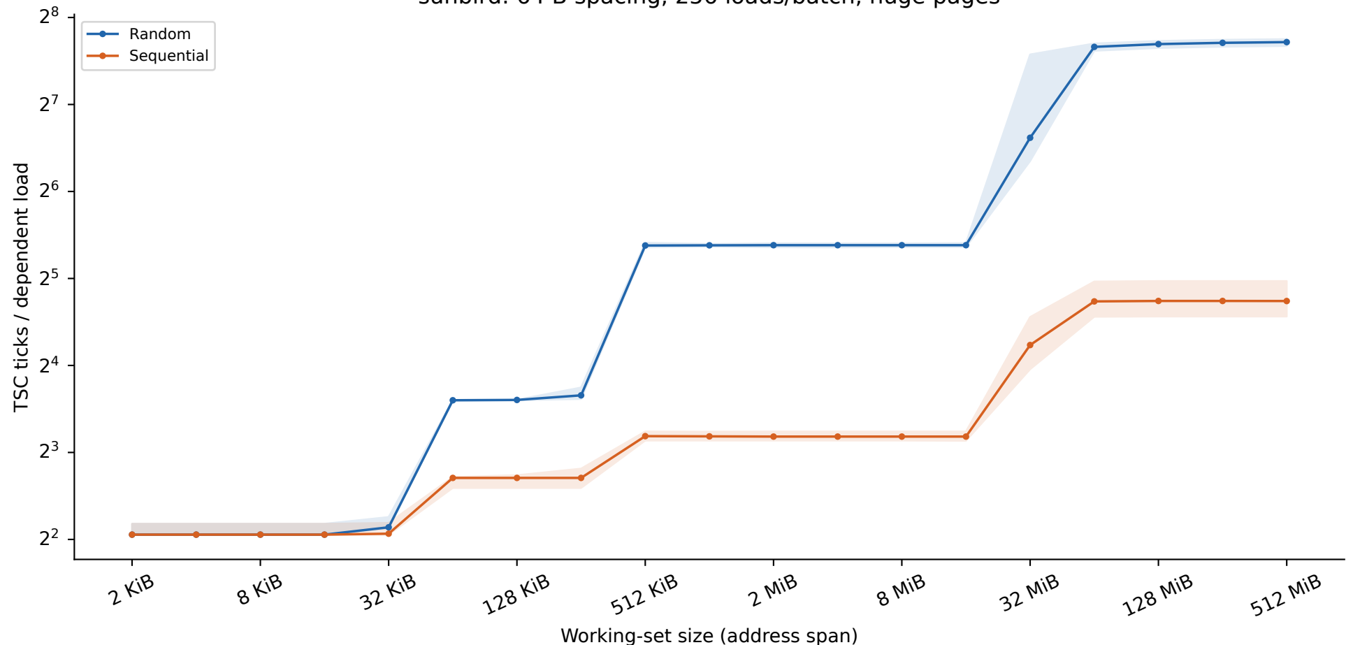
sunbird: 64 B spacing, 256 loads/batch, huge pages
