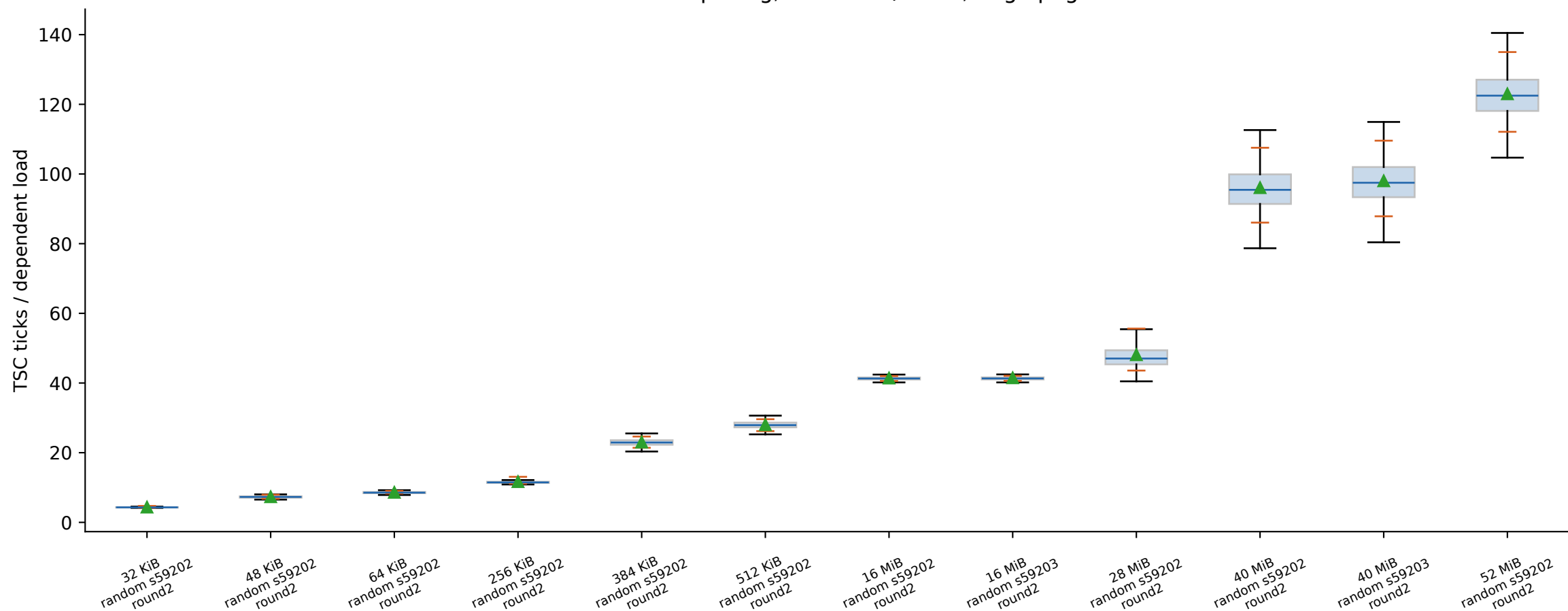
sunbird: 8 B spacing, 256 loads/batch, huge pages
