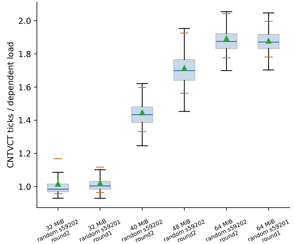
thunderbird: LLC effective transition
