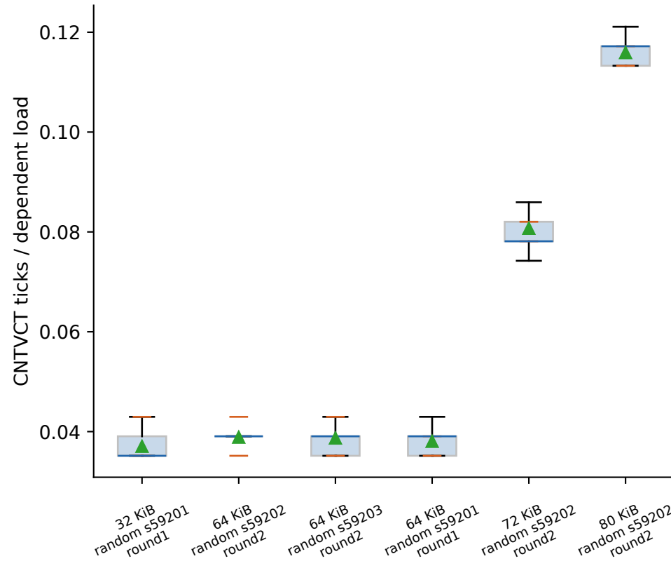
thunderbird: L1D (~64 KiB)
