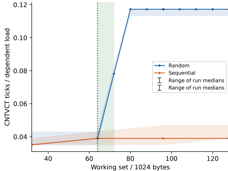
thunderbird: L1D (~64 KiB)
