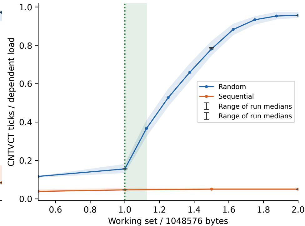
thunderbird: L2 (~1 MiB)
