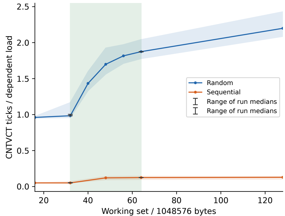
thunderbird: LLC effective transition
