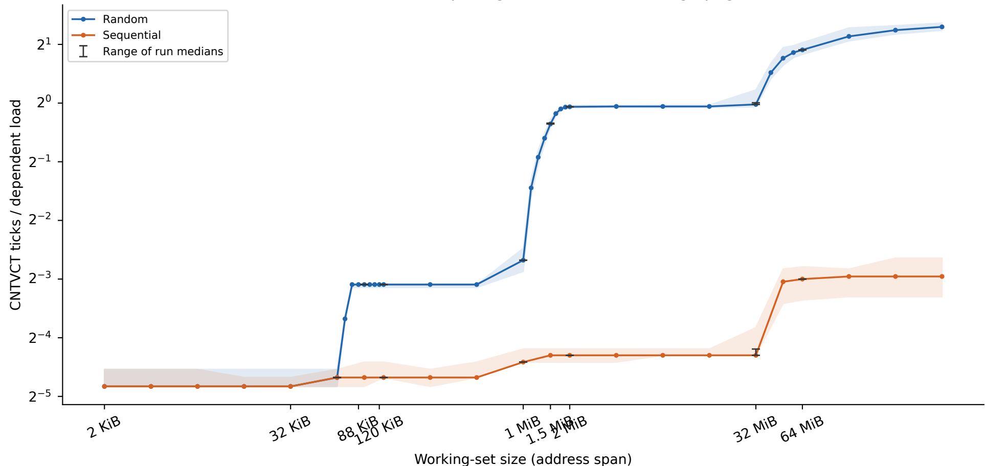
thunderbird: 64 B spacing, 256 loads/batch, huge pages
