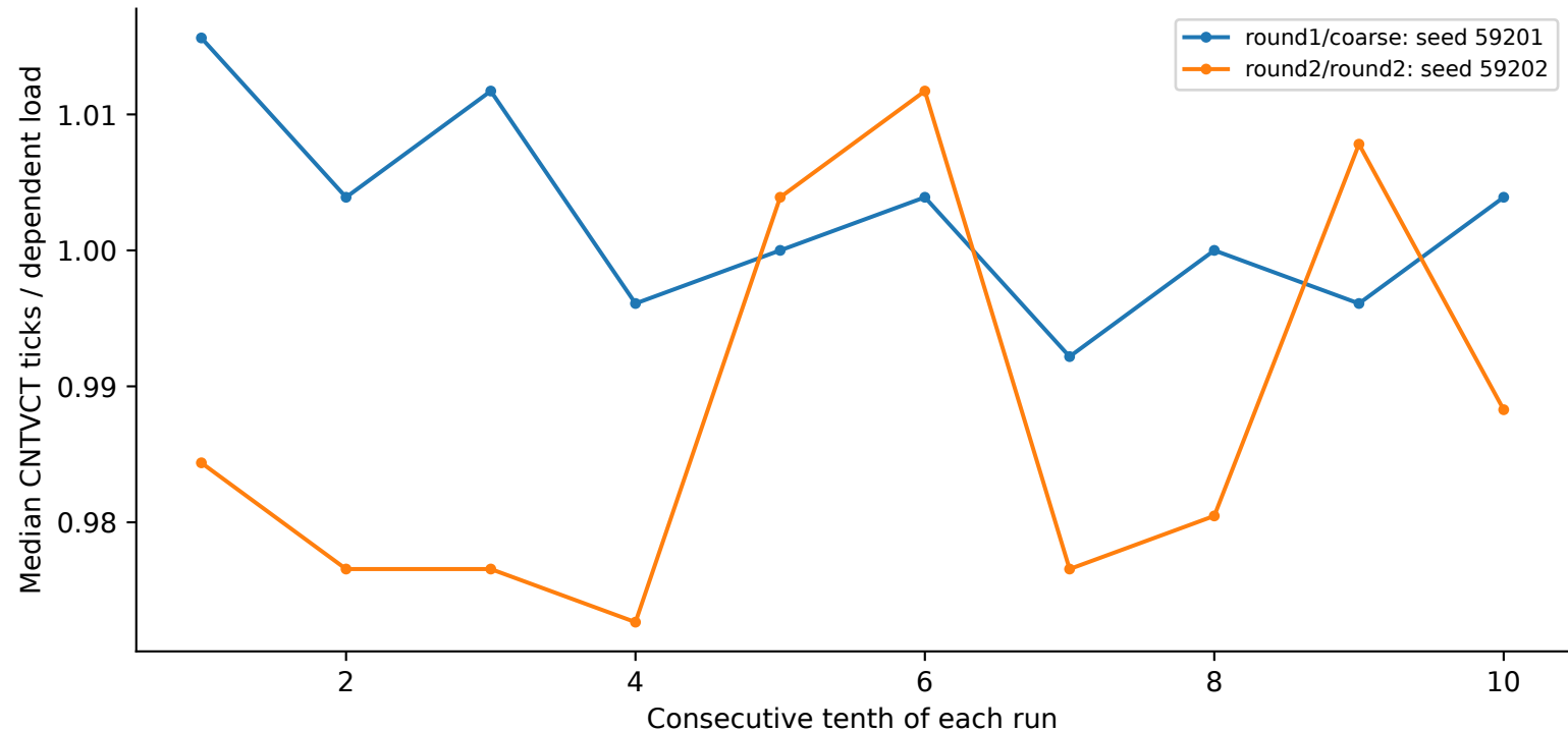
thunderbird: 32 MiB, 64 B spacing, N=256, huge
