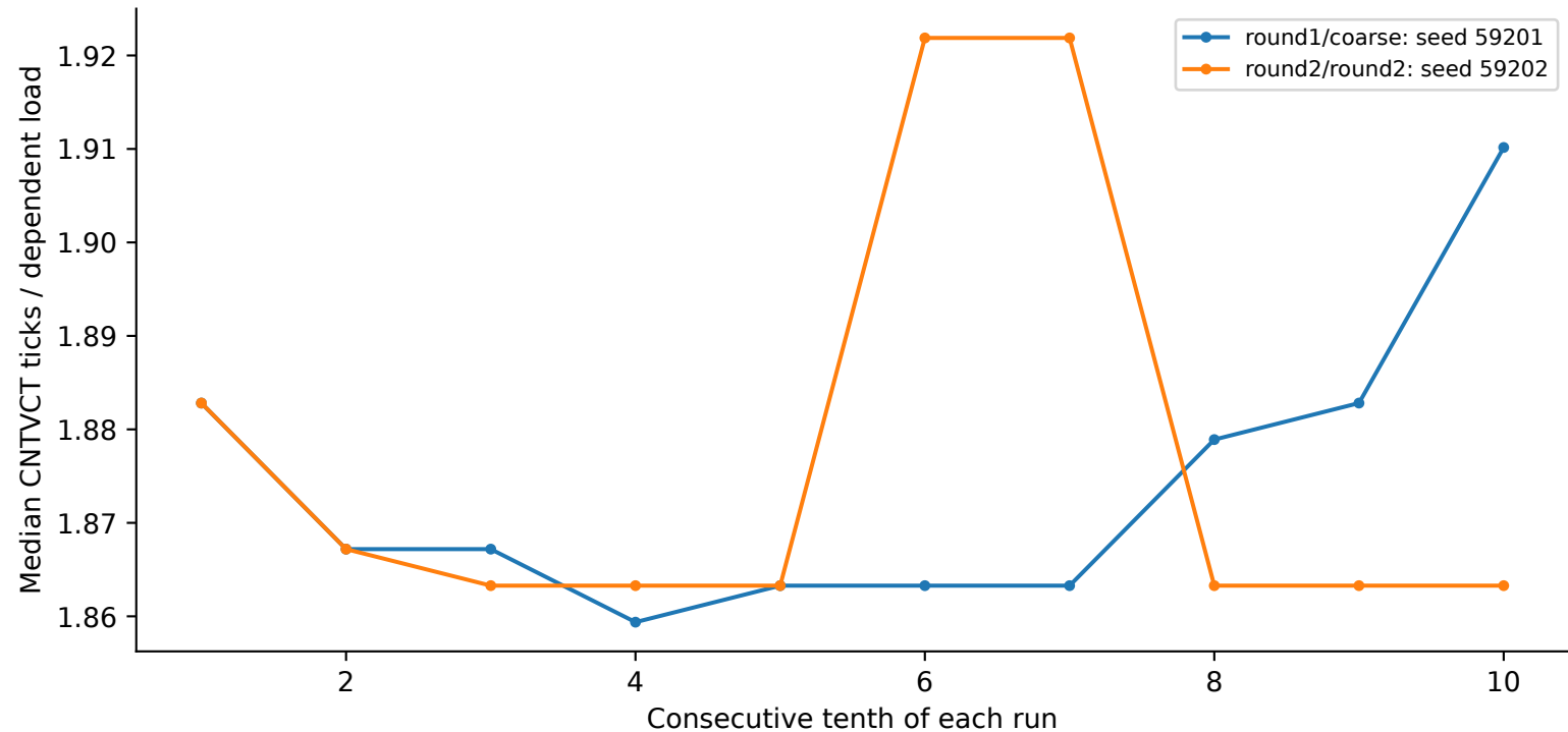
thunderbird: 64 MiB, 64 B spacing, N=256, huge
