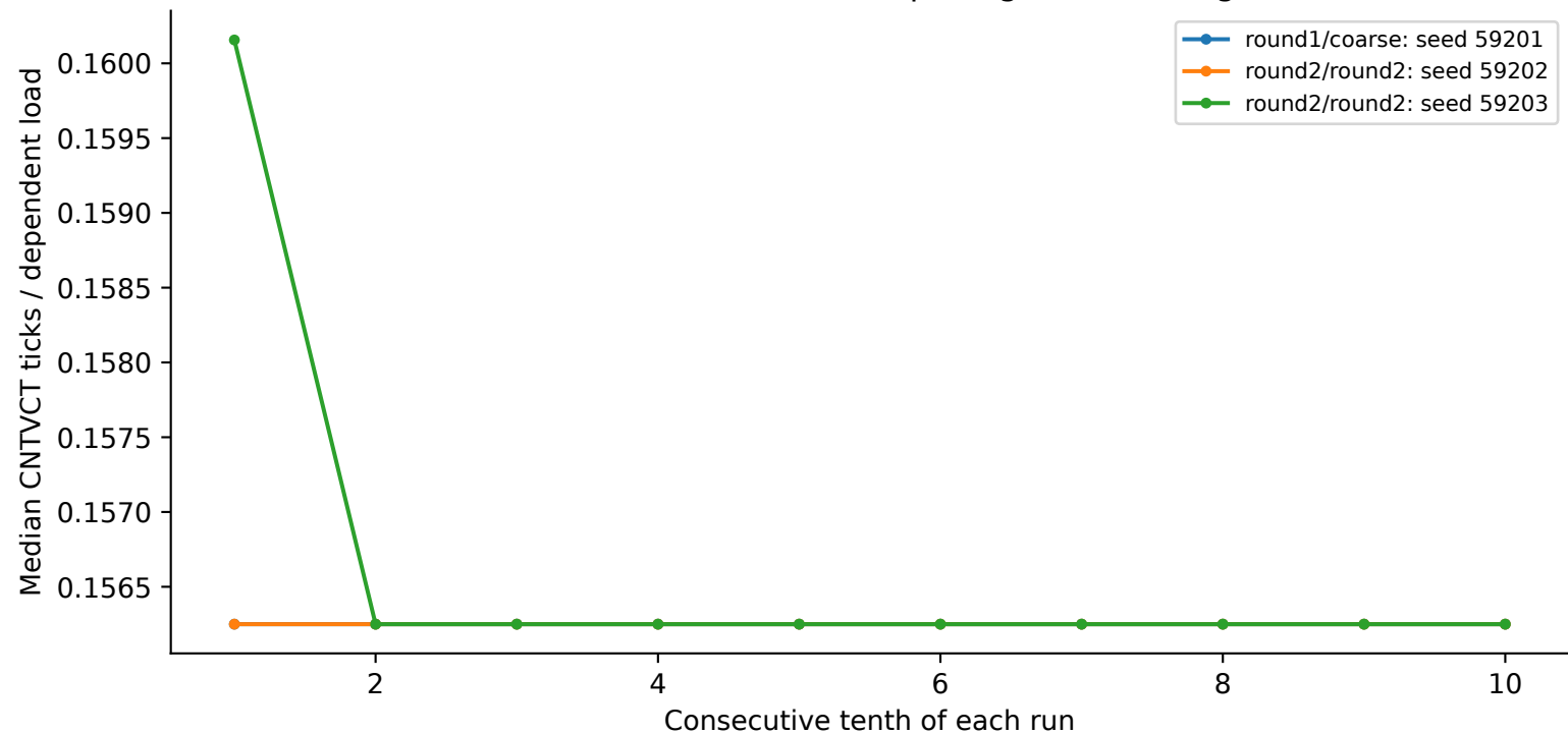
thunderbird: 1 MiB, 64 B spacing, N=256, huge
