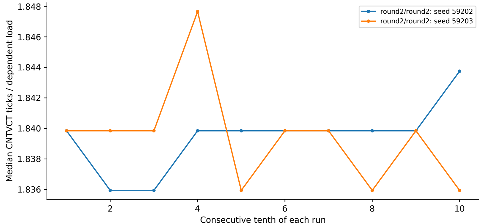
thunderbird: 64 MiB, 8 B spacing, N=256, huge
