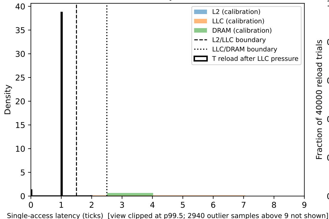
artemisia: reload latency vs. calibrated classes
