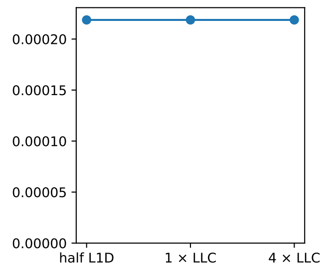
L1-dcache-stores
