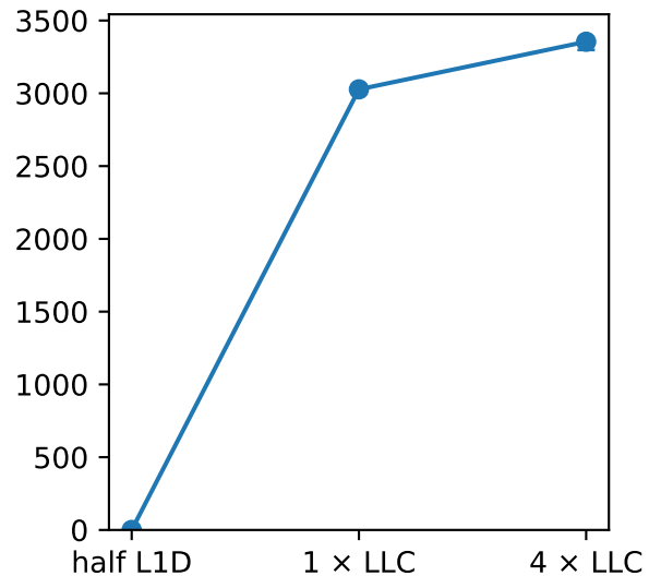
L1-dcache-stores
