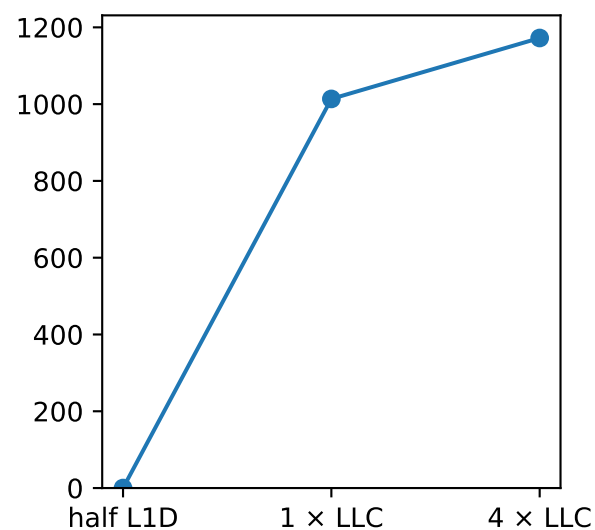
LLC-loads
