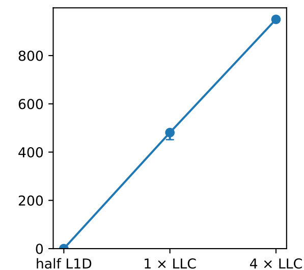
LLC-load-misses
