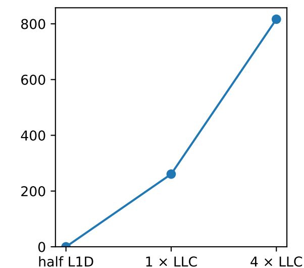
dTLB-load-misses
