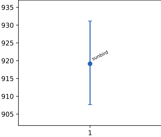
l1 loads
