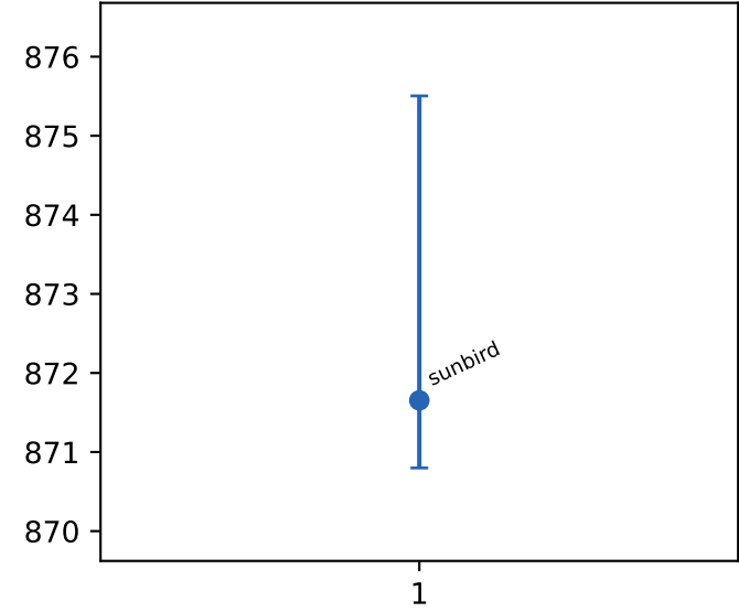
dtlb misses
