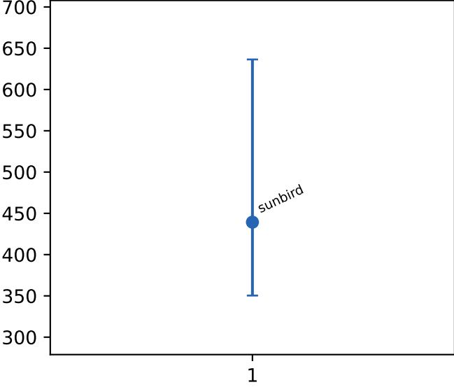
cache misses
