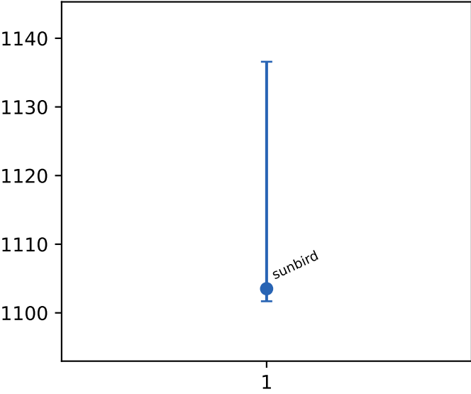
l1c loads
