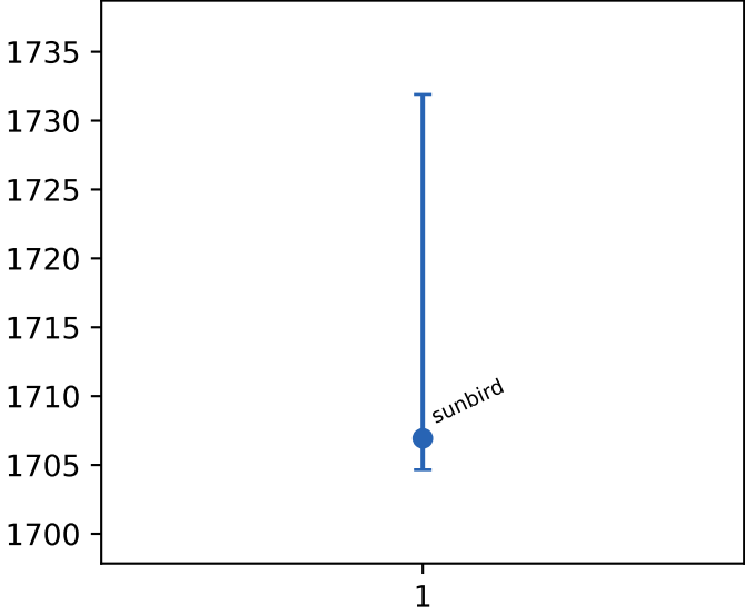
l1 misses
