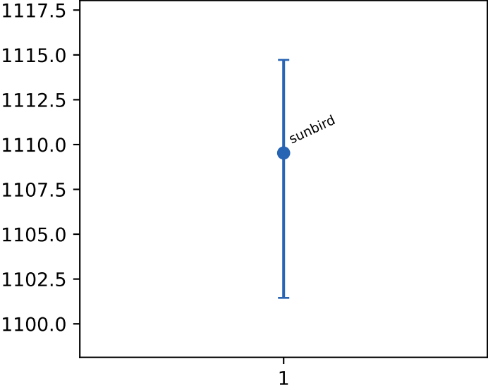
cache references
