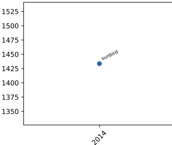
llc loads
