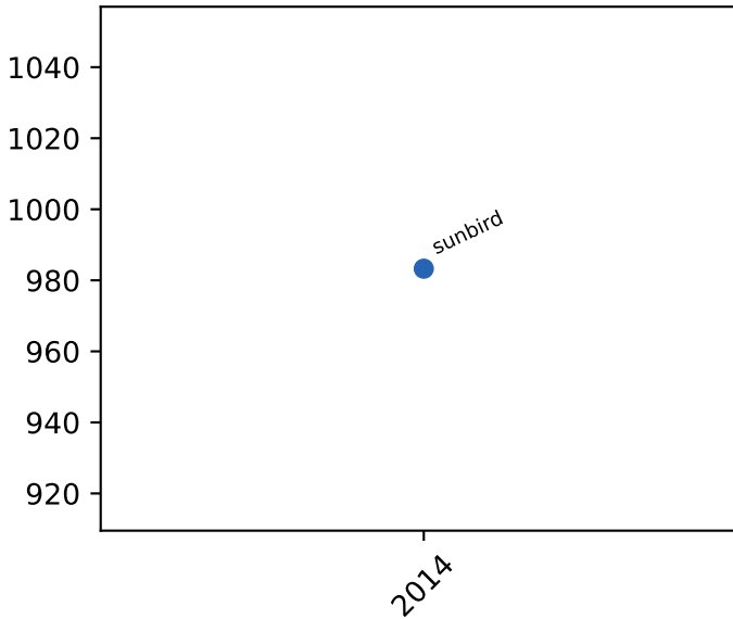
cache misses
