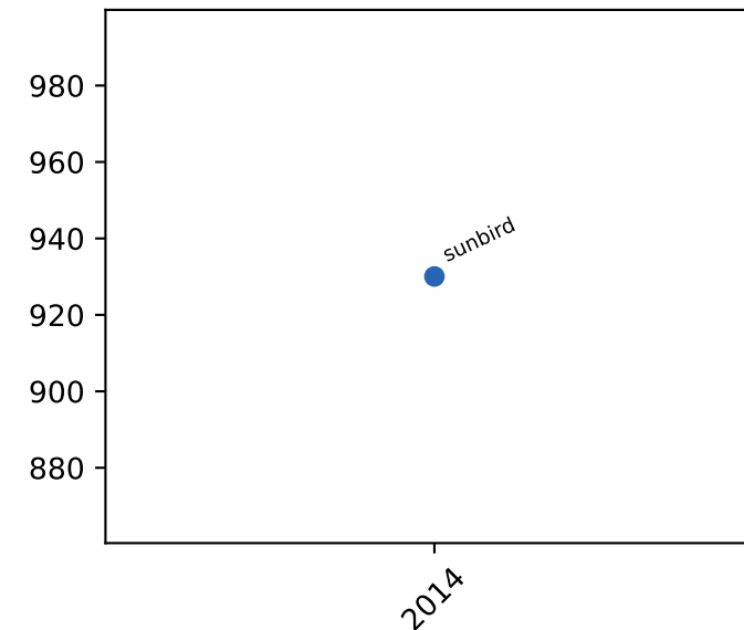
llc misses
