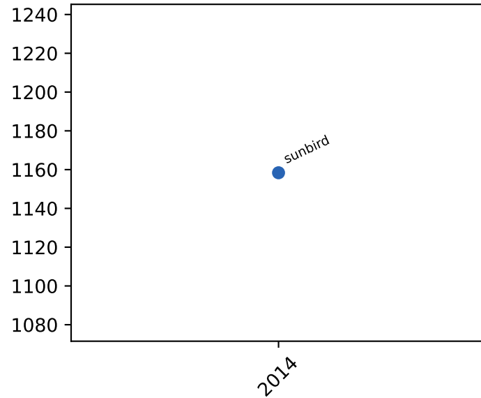
cache references
