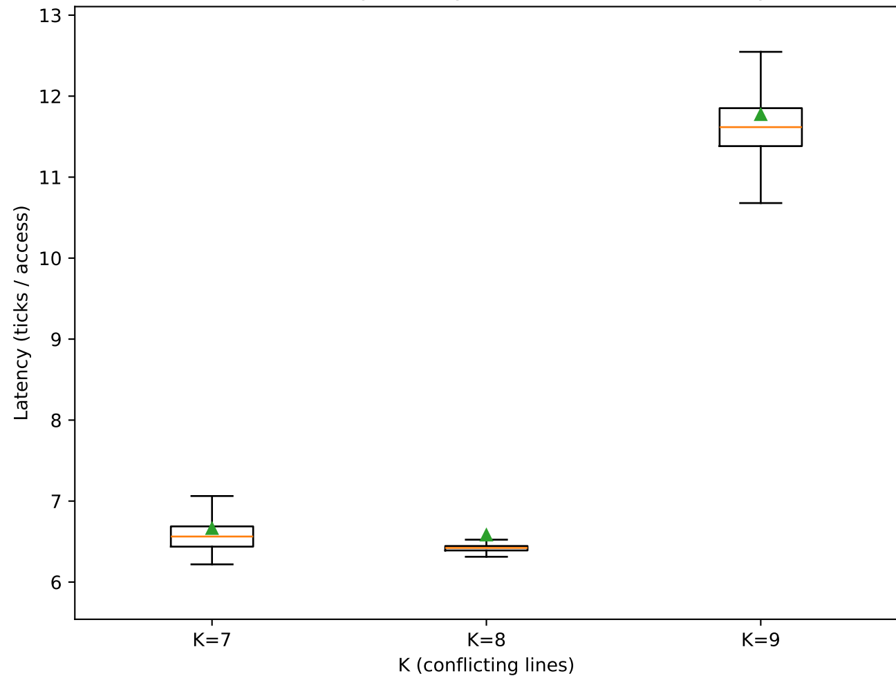
L2 associativity: latency distribution near boundary
