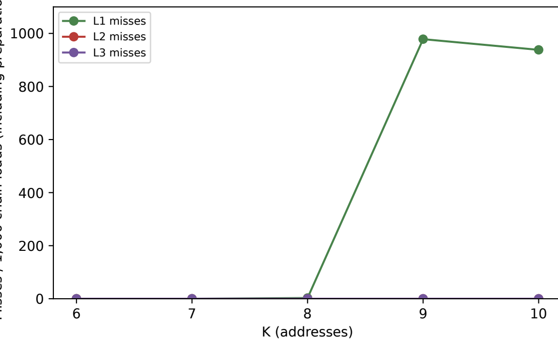
Misses / 1,000 chain loads (including preparation)
