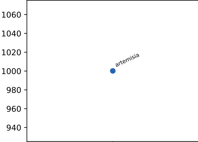
l1 loads
