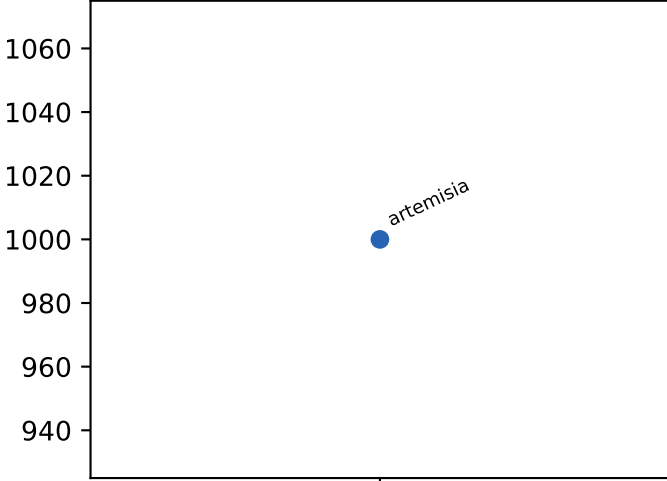
llc misses
