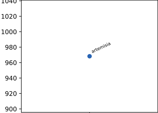
dtlb misses
