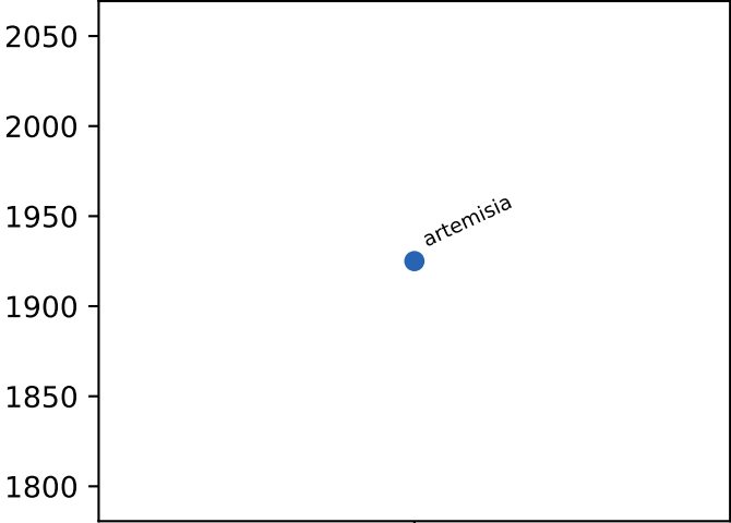
l1 misses
