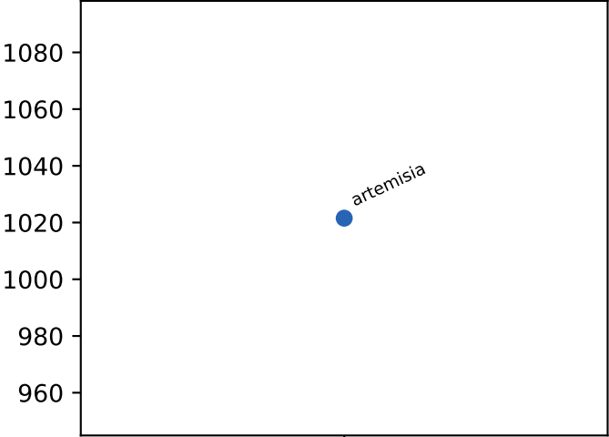
cache references
