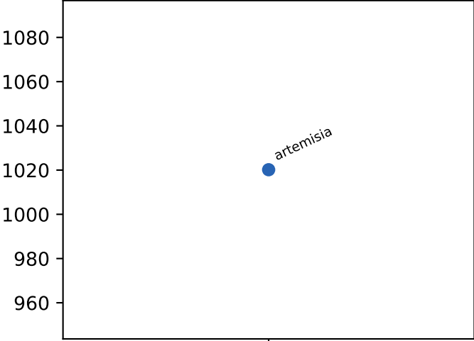
llc loads
