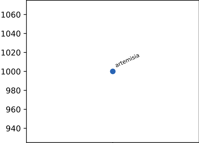
cache misses
