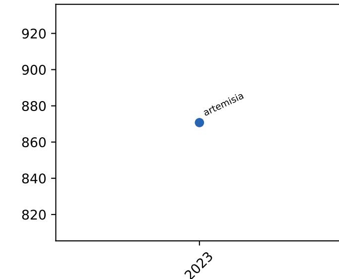
dtlb misses
