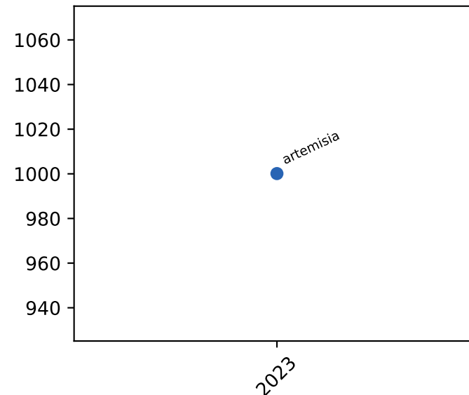
l1c loads
