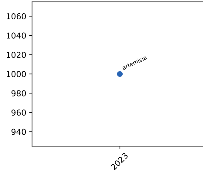
cache misses
