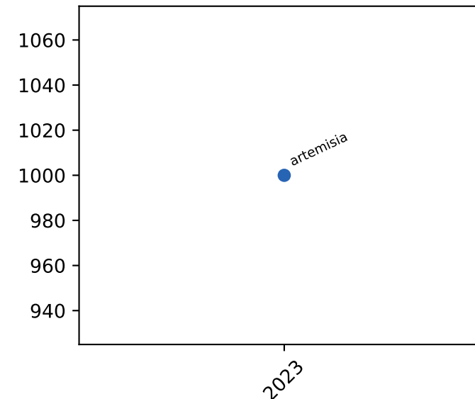
l1c misses
