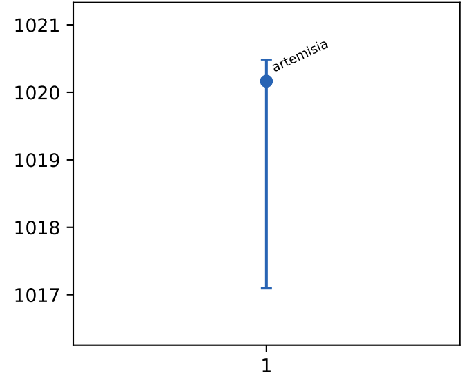
llc loads
