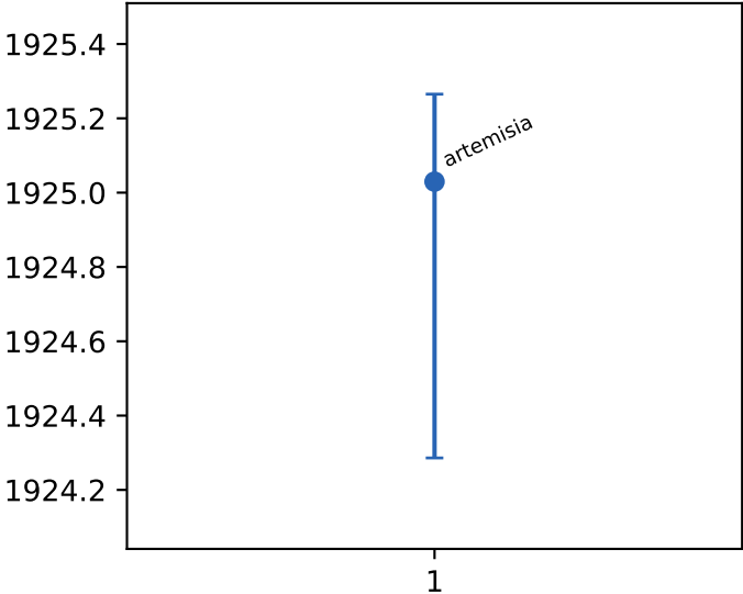
l1 misses
