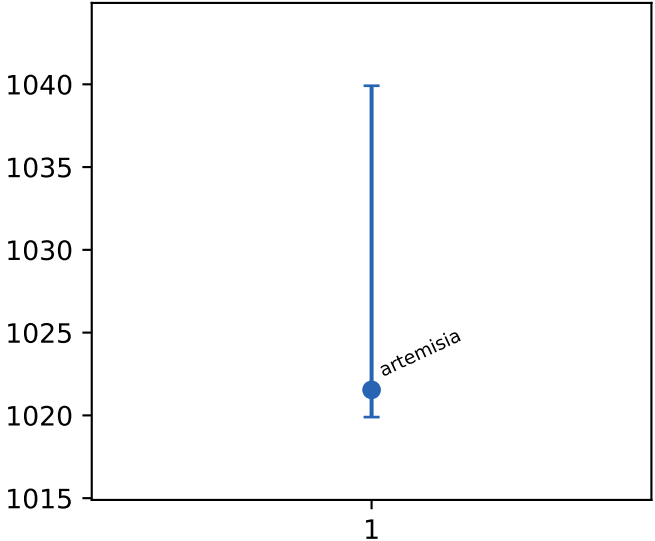
cache references
