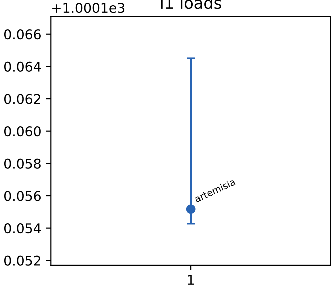
l1 loads
