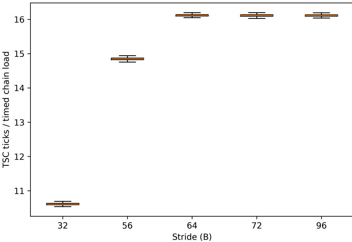
Random windows, offset 0 B
