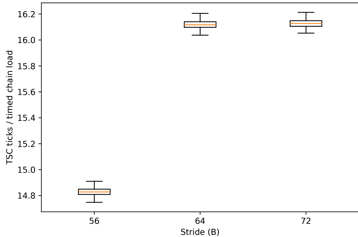
Random windows, offset 16 B
