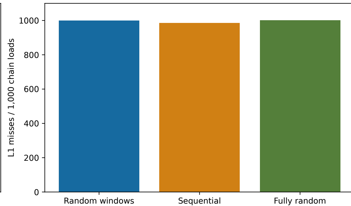
Traversal controls at 64 B stride
