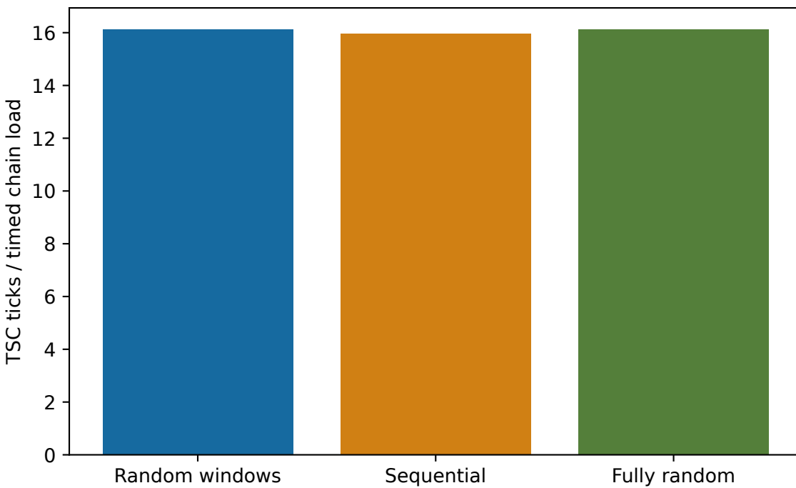
Traversal controls at 64 B stride
