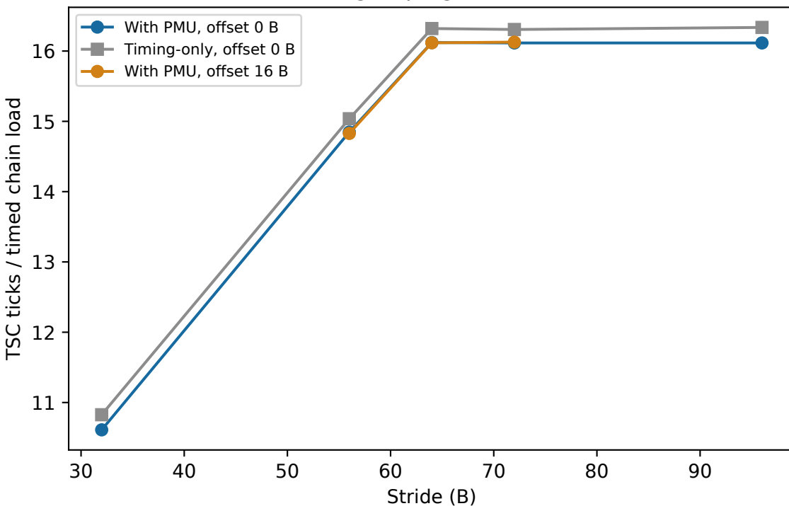
Traversal controls at 64 B stride
