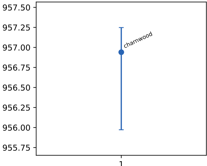
llc misses
