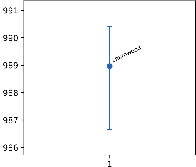
l1 loads
