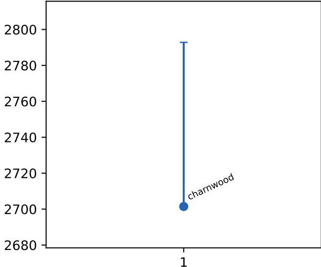
cache misses
