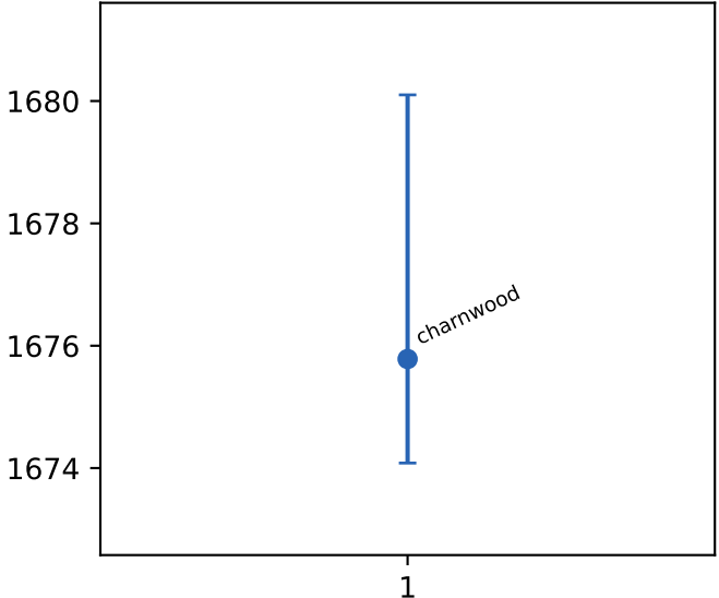
l1 misses
