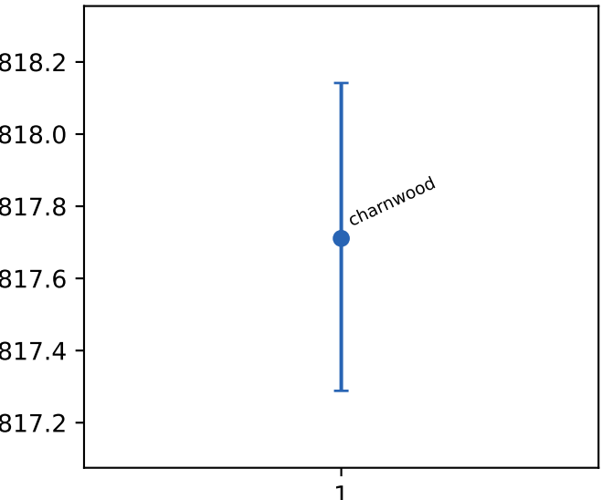
dtlb misses
