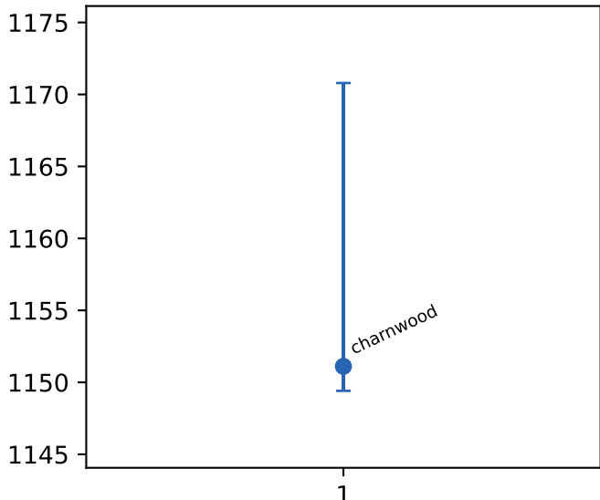
llc loads
