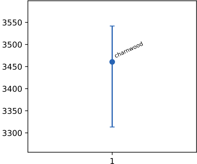
cache references
