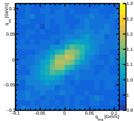
CF at charge=pos, centrality=0-10, y=[-1.00,-0.80] out-long
