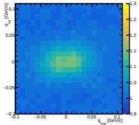
CF at charge=pos, centrality=0-10, y=[-0.20,0.00] out-long
