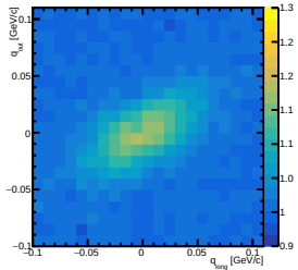
CF at charge=pos, centrality=0-10, y=[-0.80,-0.60] out-long
