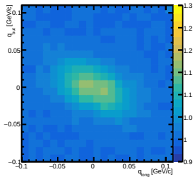
CF at charge=pos, centrality=0-10, y=[0.40,0.60] out-long
