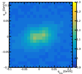
CF at charge=pos, centrality=0-10, y=[-0.40,-0.20] out-long
