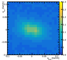
CF at charge=pos, centrality=0-10, y=[0.20,0.40] out-long
