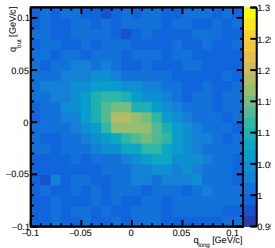
CF at charge=pos, centrality=0-10, y=[0.60,0.80] out-long
