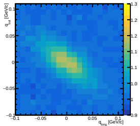
CF at charge=pos, centrality=0-10, y=[0.80,1.00] out-long
