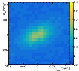
CF at charge=pos, centrality=0-10, y=[-0.60,-0.40] out-long
