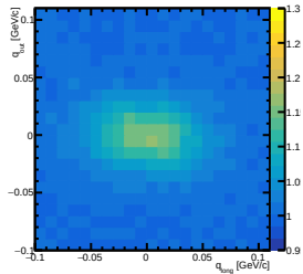
CF at charge=pos, centrality=0-10, y=[0.00,0.20] out-long
