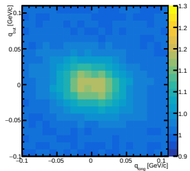
CF at charge=neg, centrality=10-30, y=[0.20,0.40] out-long
