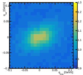
CF at charge=neg, centrality=10-30, y=[-0.60,-0.40] out-long
