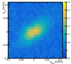
CF at charge=neg, centrality=10-30, y=[-1.00,-0.80] out-long
