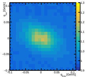
CF at charge=neg, centrality=10-30, y=[0.40,0.60] out-long
