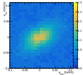
CF at charge=neg, centrality=10-30, y=[-0.80,-0.60] out-long
