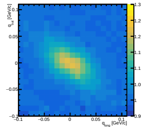
CF at charge=neg, centrality=10-30, y=[0.80,1.00] out-long
