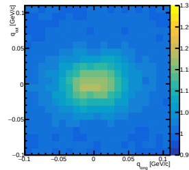
CF at charge=neg, centrality=10-30, y=[-0.20,0.00] out-long
