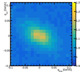
CF at charge=neg, centrality=10-30, y=[0.60,0.80] out-long
