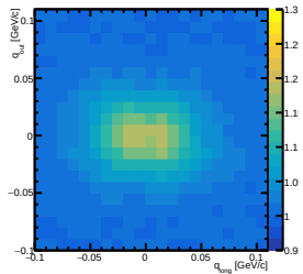
CF at charge=neg, centrality=10-30, y=[0.00,0.20] out-long
