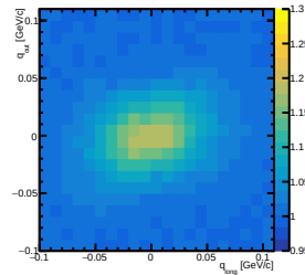
CF at charge=neg, centrality=10-30, y=[-0.40,-0.20] out-long
