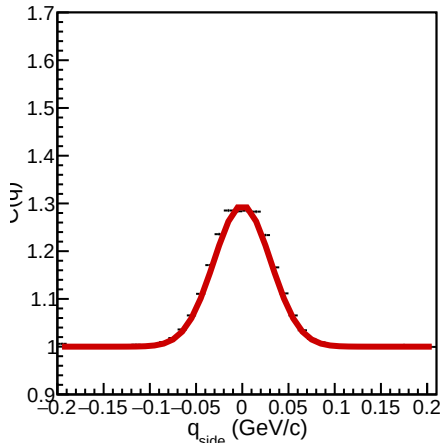
CF at charge=neg, centrality=0-10, y=[0.00,0.20] side
