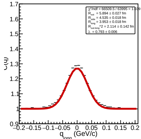
CF at charge=neg, centrality=0-10, y=[0.00,0.20] long
