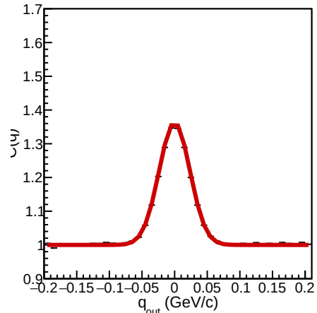
CF at charge=neg, centrality=0-10, y=[0.00,0.20] out
