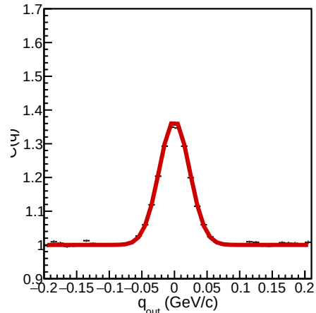
CF at charge=pos, centrality=0-10, y=[0.00,0.20] out
