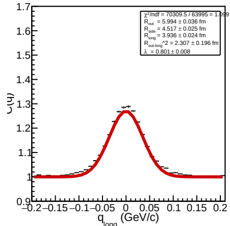
CF at charge=pos, centrality=0-10, y=[0.00,0.20] long
