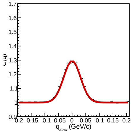
CF at charge=pos, centrality=0-10, y=[0.00,0.20] side
